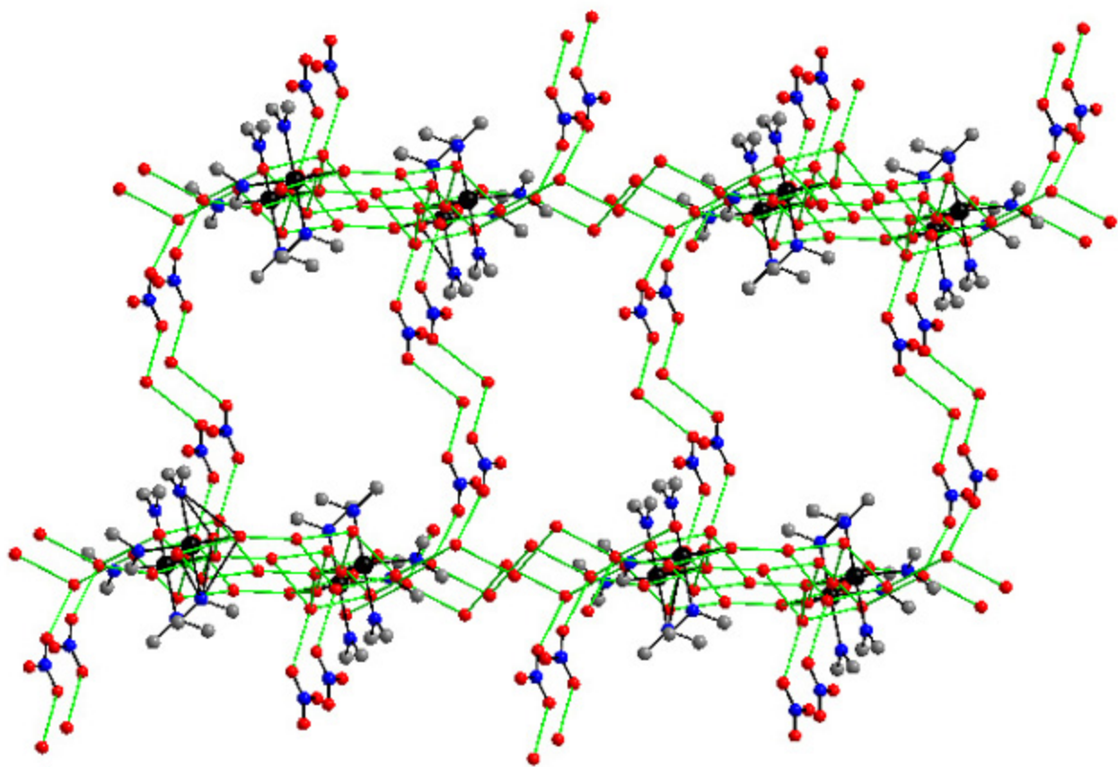
S-1. Assembly of water molecules with nitrate anions in compound 2 .
