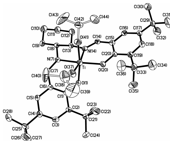
Fig. S1 The molecular structure of 6 (40% probability ellipsoids).
