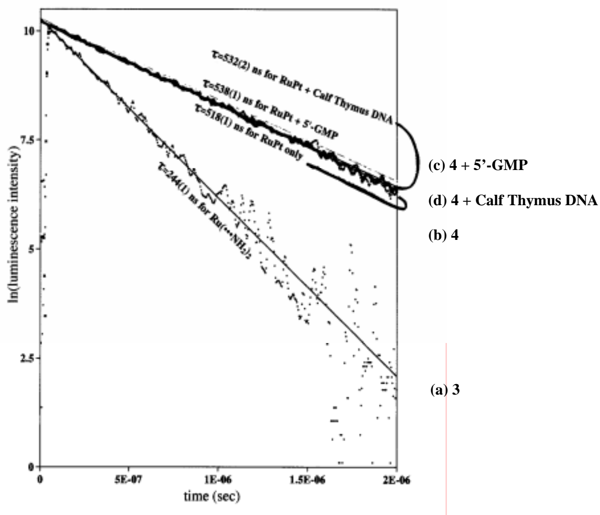
Figure S1. Luminescence decays observed for aqueous solutions of (a) 3 , (b) 4 , (c) 4 and 5'-GMP, (d) 4 and Calf Thymus DNA in air at room temperature. Experimental conditions are same to those given in Figures 3 and 4 reported in the main text.
