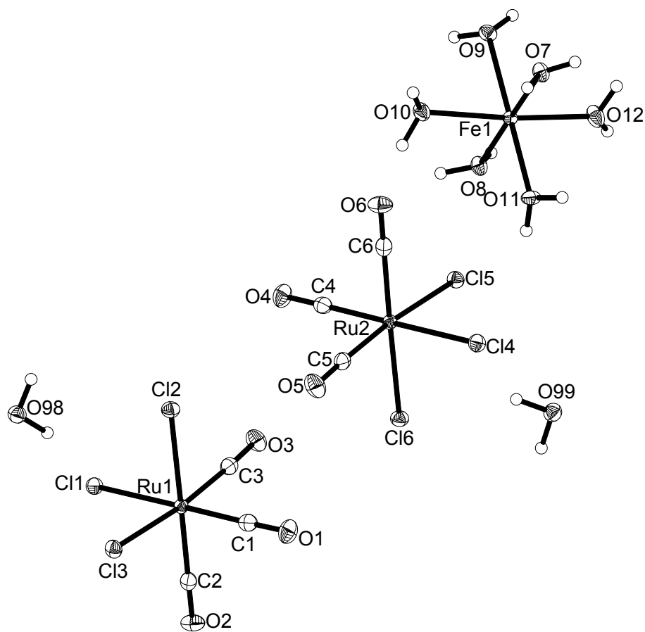
Thermal ellipsoid plot of 1c .
