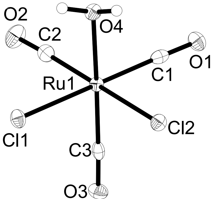
Thermal ellipsoid plot of 3 .
