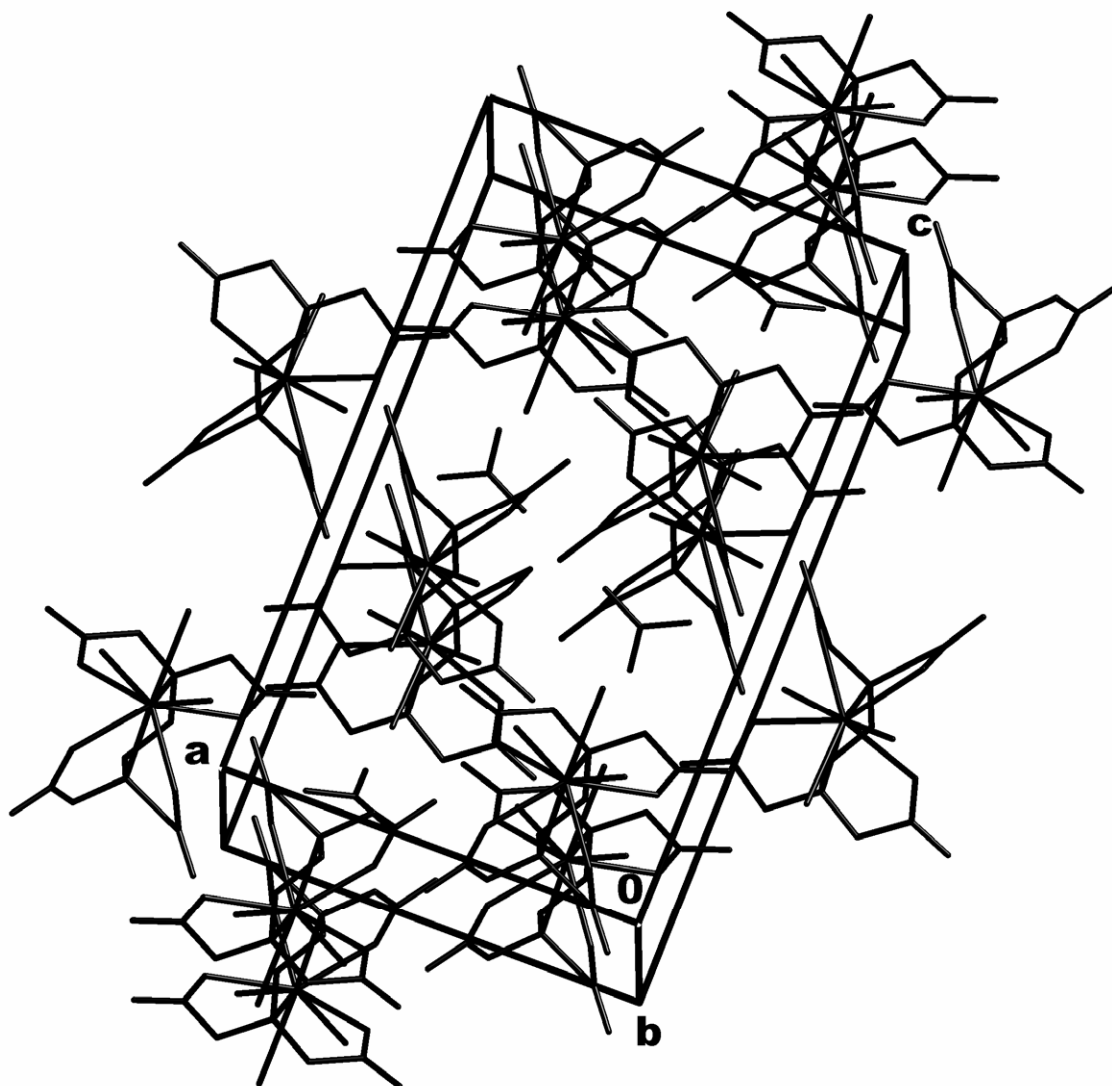
Figure S1B. A view of the unit cell of [C(NH 2 ) 3 ][Eu(EDTA)(H 2 O) 3 ].
