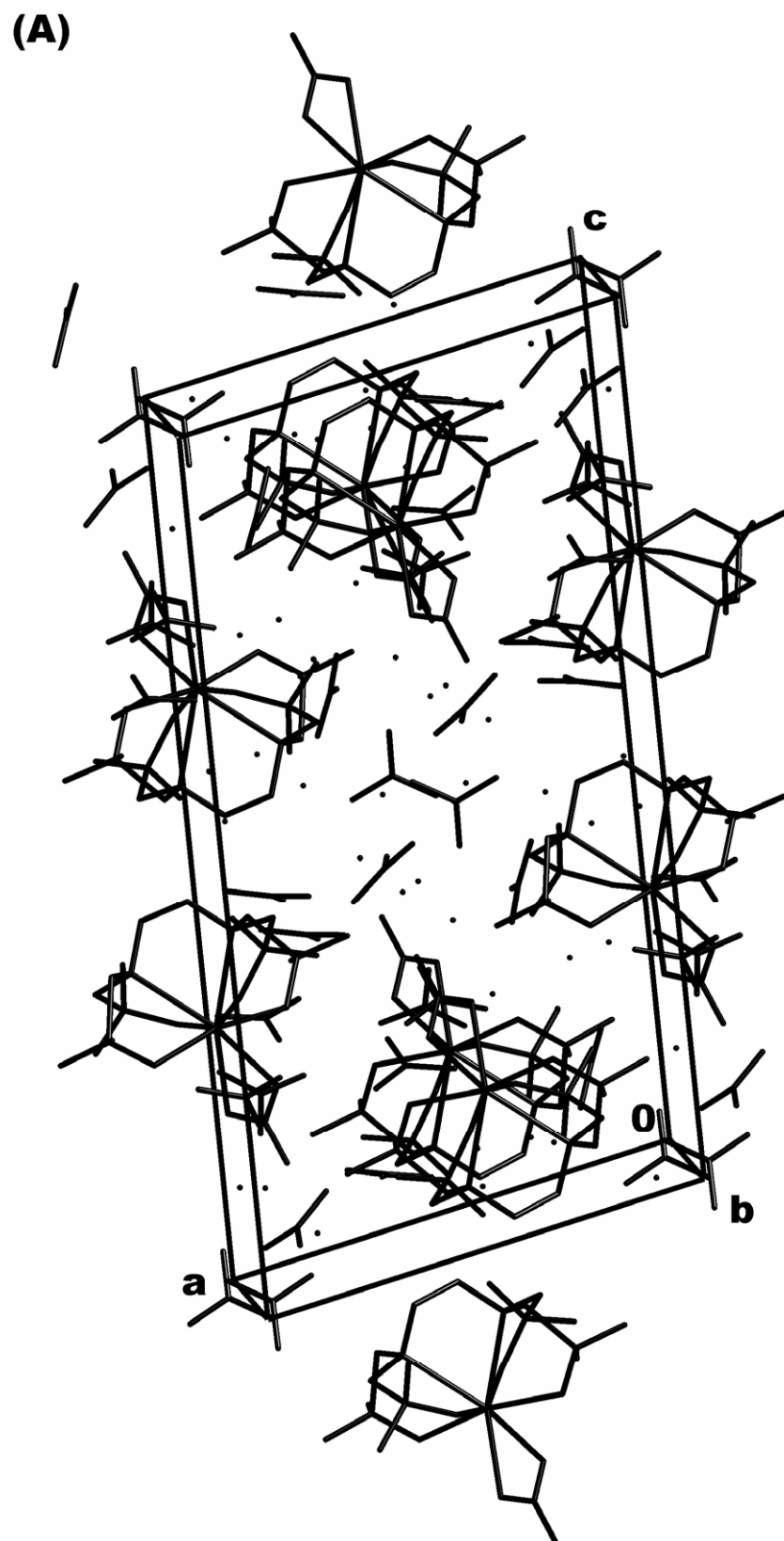
Figure S1A. A view of the unit cell of [\text{C}(\text{NH}_2)_3]_7[\text{Eu}(\text{EDTMP})(\text{CO}_3)] \cdot 10\text{H}_2\text{O} .
