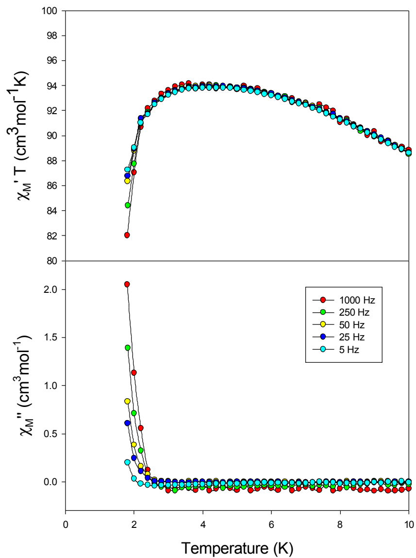
Figure SI2. Plots of the in-phase ( \chi_M' ) signal as \chi_M' T and out-of-phase ( \chi_M'' ) signal in ac susceptibility studies vs. temperature for 1 in a 3.5 G field oscillating at the indicated frequencies.
