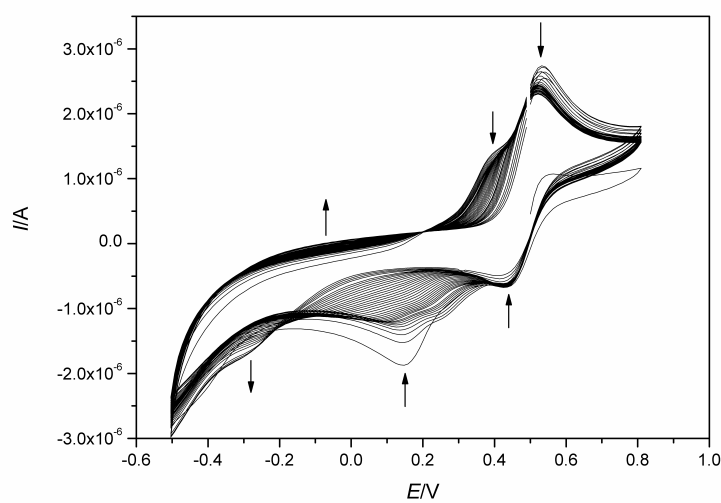
Supplementary information fig. 3. Cyclic voltammograms of the complex 4 in DMSO under aerobic condition. Ferrocene was added as internal standard, being observed near 0.4 V.
