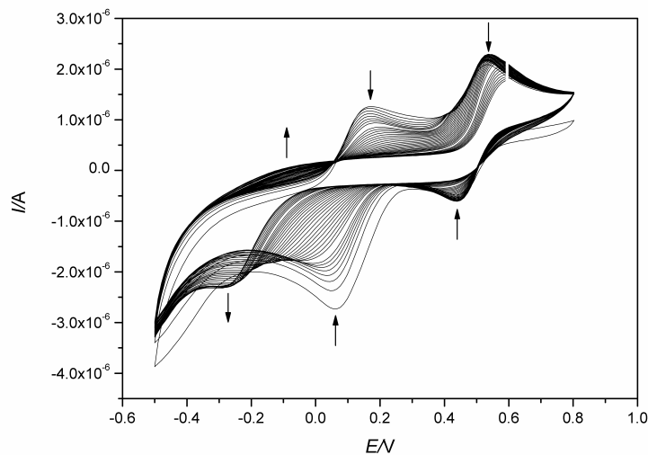
Supplementary information fig. 2 Cyclic voltammograms of the complex 3 in DMSO under aerobic condition. Ferrocene was added as internal standard, being observed near 0.4 V.
