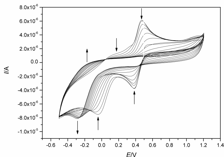
Supplementary information fig. 1 Cyclic voltammograms of the complex 1 in CH 3 CN under aerobic condition. Ferrocene was added as internal standard, being observed near 0.4 V.
