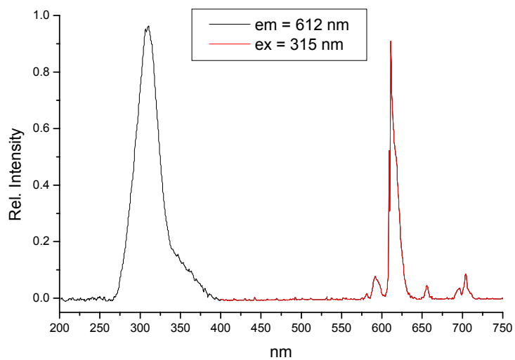
Excitation and Emission spectra of a 0.146mM CH 3 CN solution of 3
