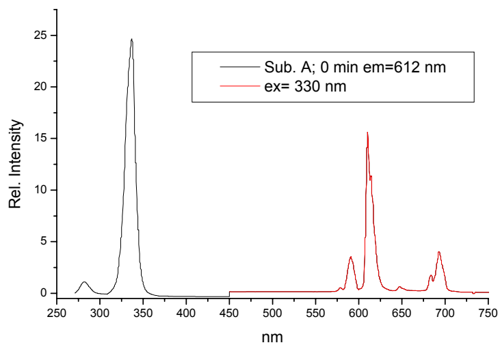
Excitation and Emission spectra of a 0.145mM CH 3 CN solution of 1
