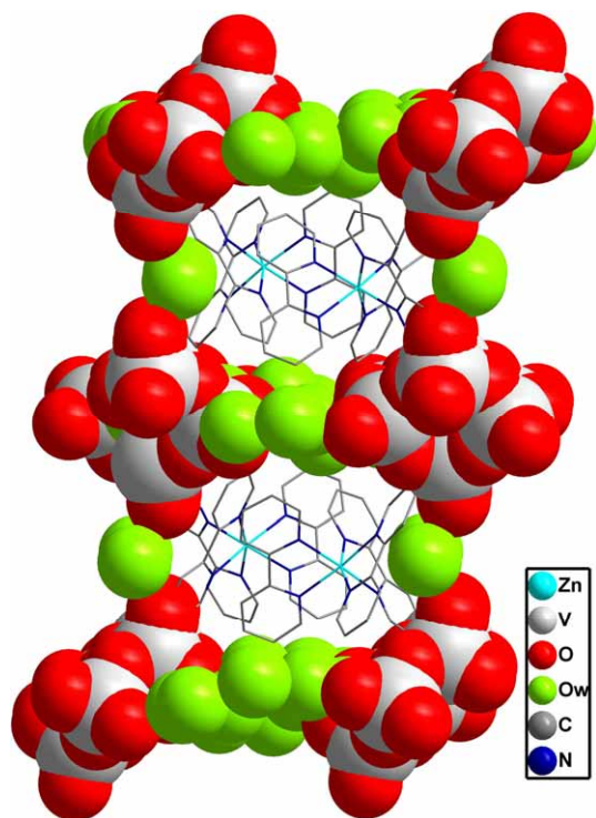
Fig. S1 The 3-D network of compound \text{Zn}(\text{2,2'}\text{-bpy})_3[\text{V}_4\text{O}_{12}] \cdot 11\text{H}_2\text{O}
