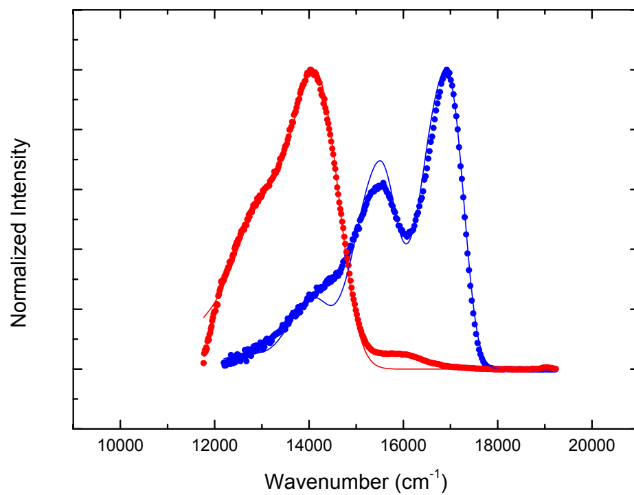
Figure S. Vibronic analysis of the luminescence profiles obtained at 77 K for the cis - ( 1a ; blue) and trans -( 1b ; red) [Ru(DIP) 2 (MeOH) 2 ][OTf] 2 complexes (experimental data, and fitted
