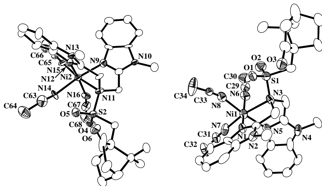
Figure S1. Thermal ellipsoid representation of complex 4 in its asymmetric cell at 50 % probability level. Hydrogen atoms, solvent molecules and the counter anions are omitted for clarity.
