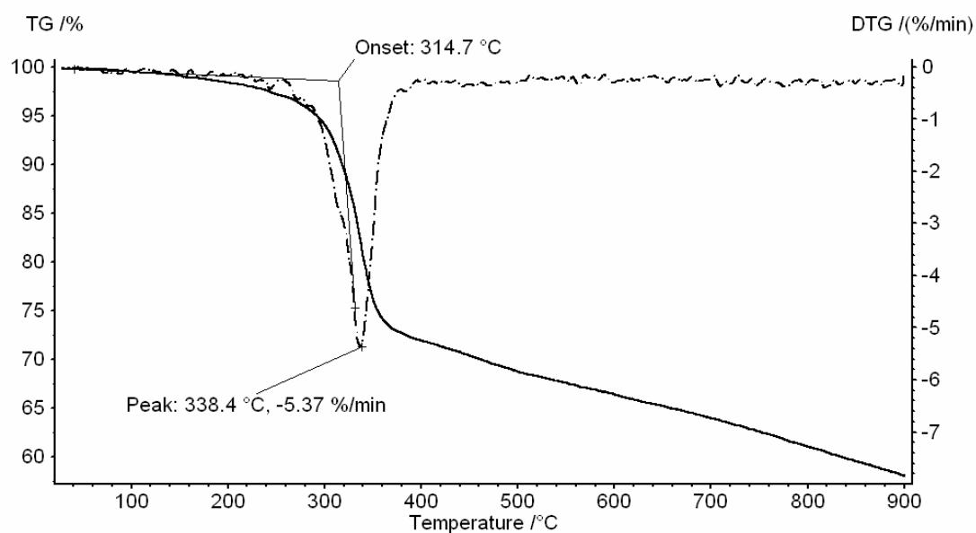
Figure S2. Thermogravimetric analysis curves of 2 under a argon atmosphere (a) TG curve (solid line); (b) DTG curve (dash dot line).
