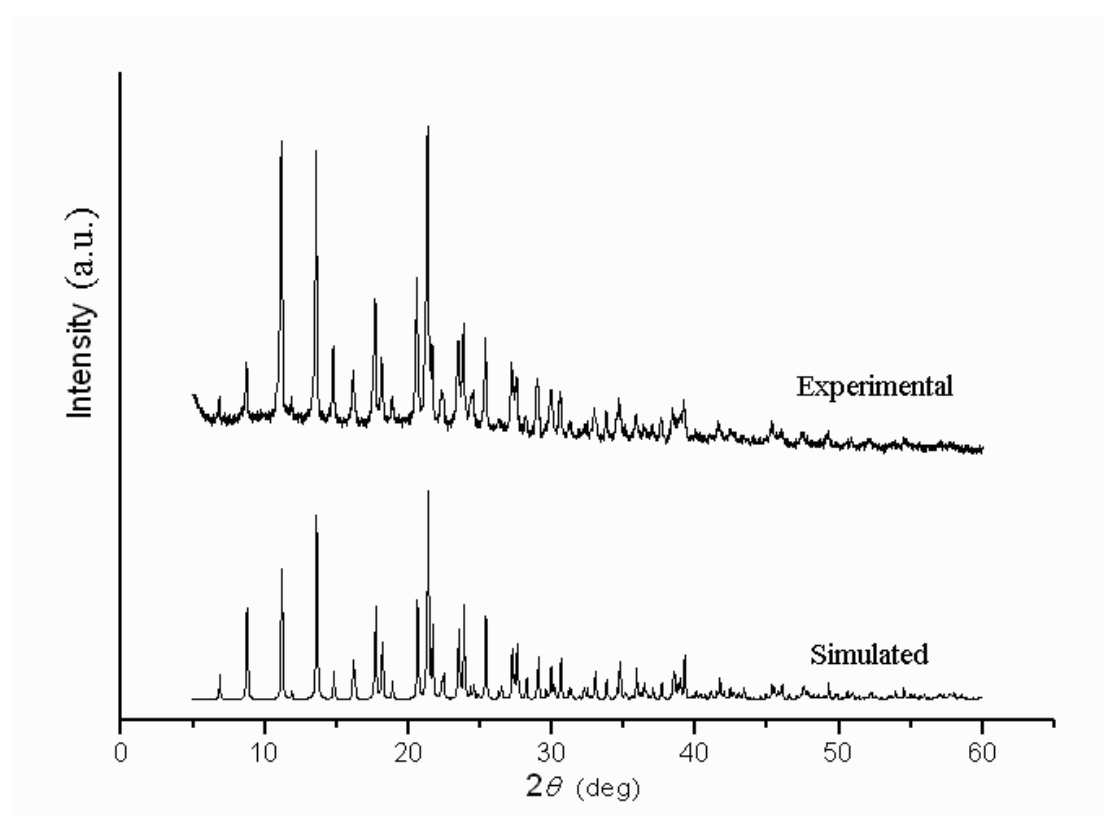
Figure S1. XPRD patterns for 2 : (a) powder diffraction pattern; (b) calculated pattern from single crystal X-ray data.
