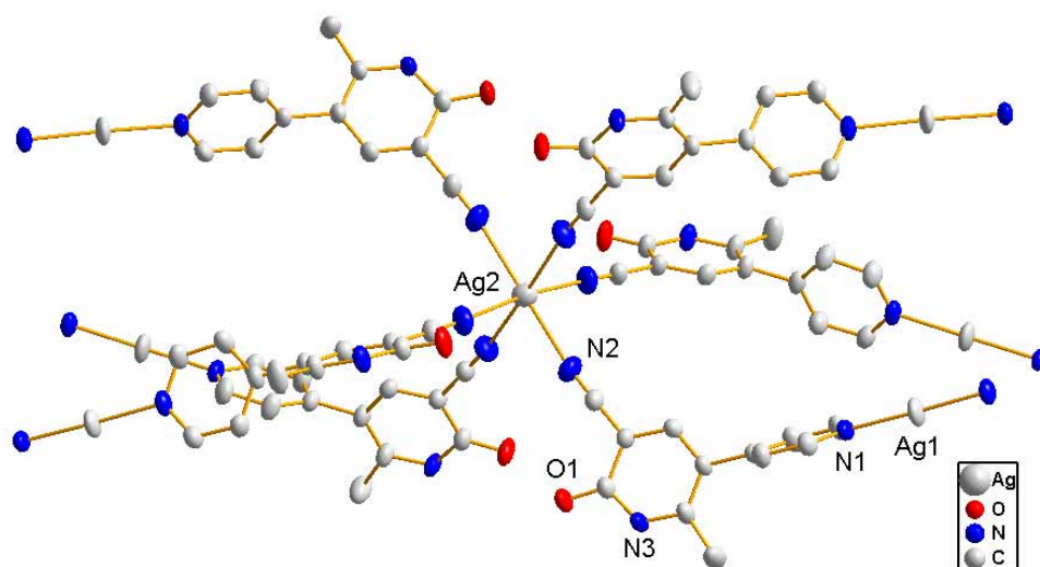
Figure S3. Partial view of the crystal structure of 2 (hydrogen atoms, methanol molecules and \text{PF}_6^- anions omitted for clarity).
