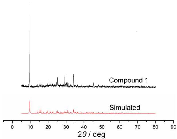
Figure S1. XRD patterns of compound 1 compared with its simulated XRD pattern from crystallographic data.
