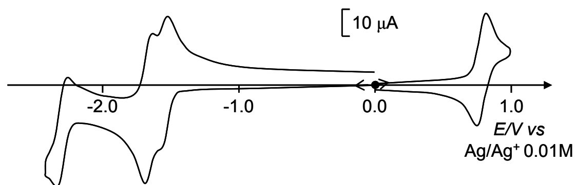
Figure S1. Cyclic voltammogram of a 0.46 mM solution of (III) in CH 3 CN + 0.05 M Bu 4 NPF 6 at a platinum electrode (0.5 cm of diameter); scan rate: 100 mV s -1 .
