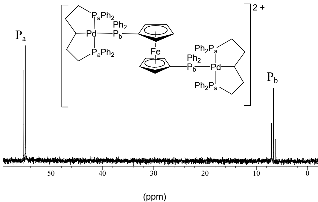
Figure S1. ^{31}\text{P}\{^1\text{H}\} NMR spectrum of complex 3 in \text{CDCl}_3
