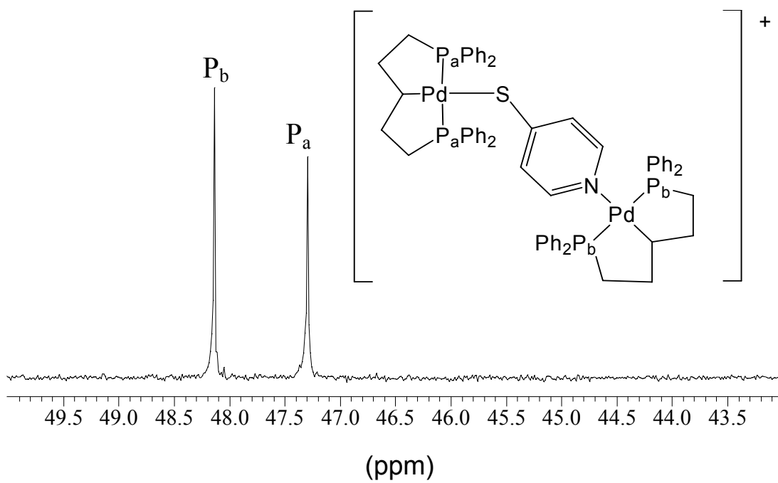
Figure S2. ^{31}\text{P}\{^1\text{H}\} NMR spectrum of complex 6 in \text{CDCl}_3
