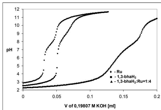
Fig. 2 Titration curves for Ru : 1,3-bhaH 2 system where Ru = K[Ru(Hedta)Cl].
