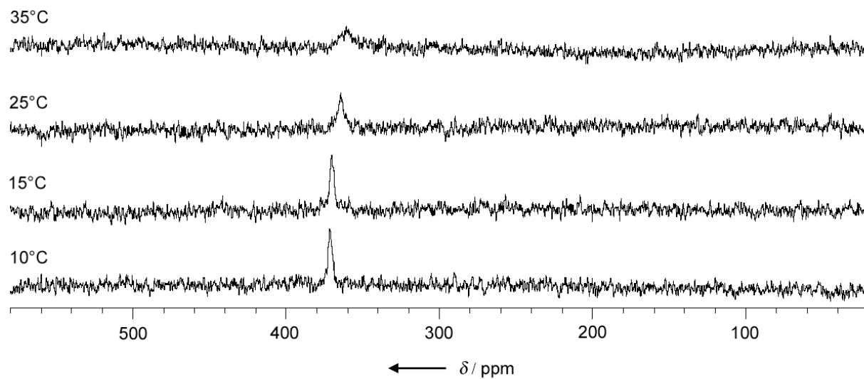
Fig. S1 VT ^{171}\text{Yb} NMR experiment of [\text{Yb}(\text{AlEt}_4)_2]_n ( 2b ).
