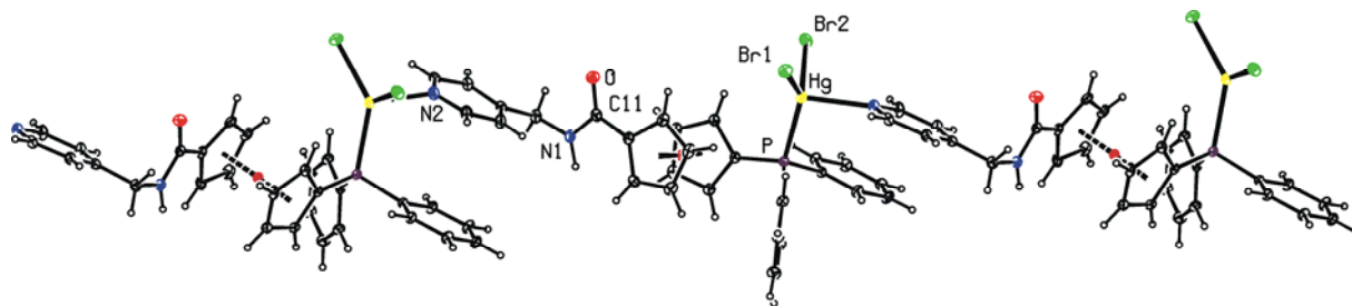
Figure S1. PLATON plot of the infinite linear polymeric chain in complex 5 . Displacement ellipsoids enclose 30% probability level.
