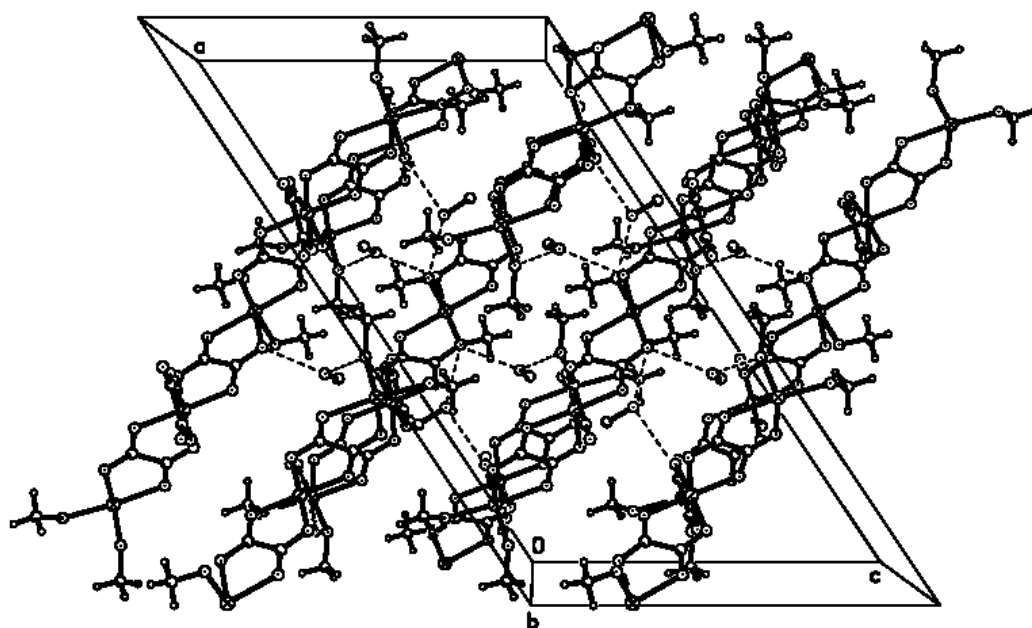
S1 Cell packing diagram along the b axis showing the planar layers in 1 .
