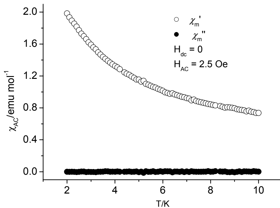
S2 Zero-static AC magnetic susceptibility under an AC magnetic field of 2.5 Oe for 1 .
