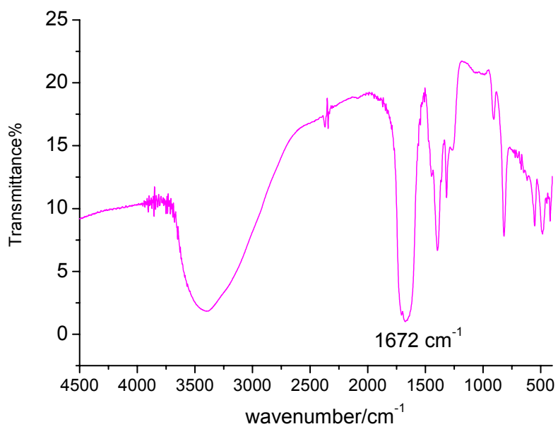
S4 IR spectrum of 1 .
