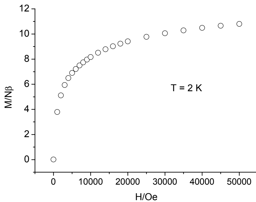
S3 Magnetisation curve at 2 K for 1 .
