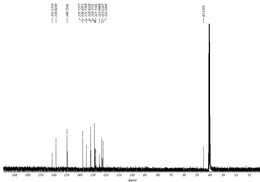
Figure 6 ^{13}\text{C} NMR Spectra of 5 in \text{DMSO-d}_6
