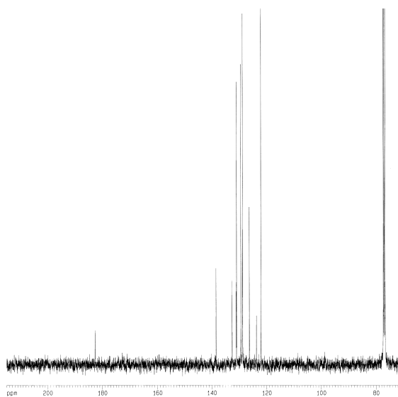
Figure 2 13 C NMR Spectra of 3 in CDCl 3
