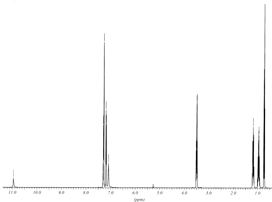
Figure 3 ^1\text{H} NMR Spectra of 4 in \text{CDCl}_3
