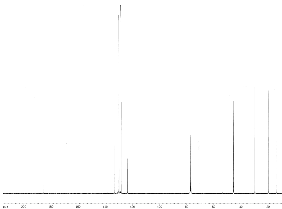
Figure 4 ^{13}\text{C} NMR Spectra of 4 in \text{CDCl}_3
