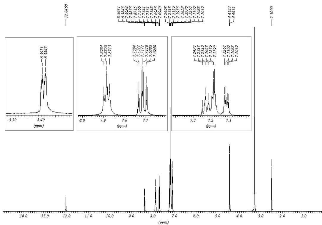
Figure 5 ^1\text{H} NMR Spectra of 5 in \text{DMSO-d}_6
