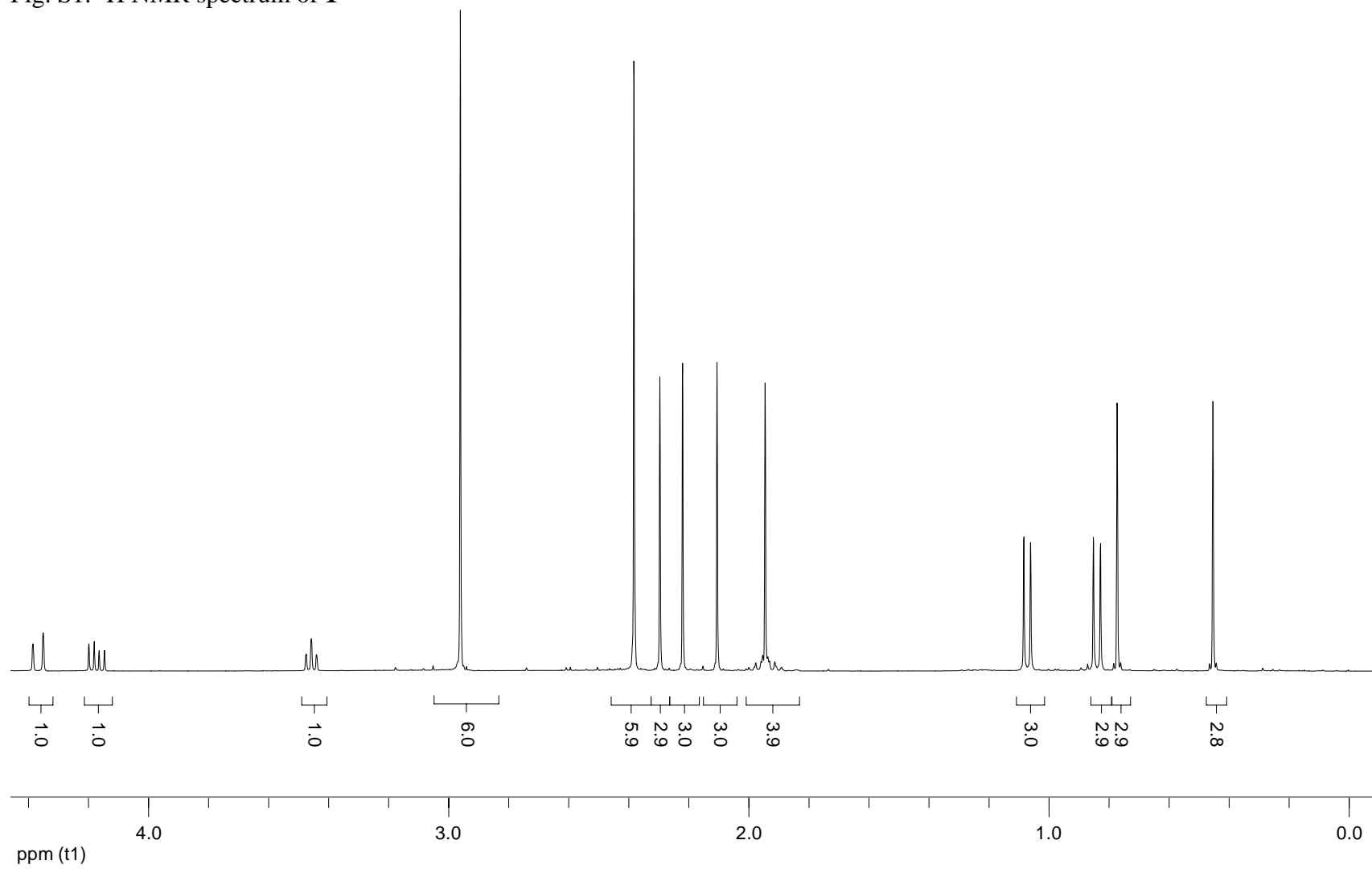
Fig. S1. ^1\text{H} NMR spectrum of 1
