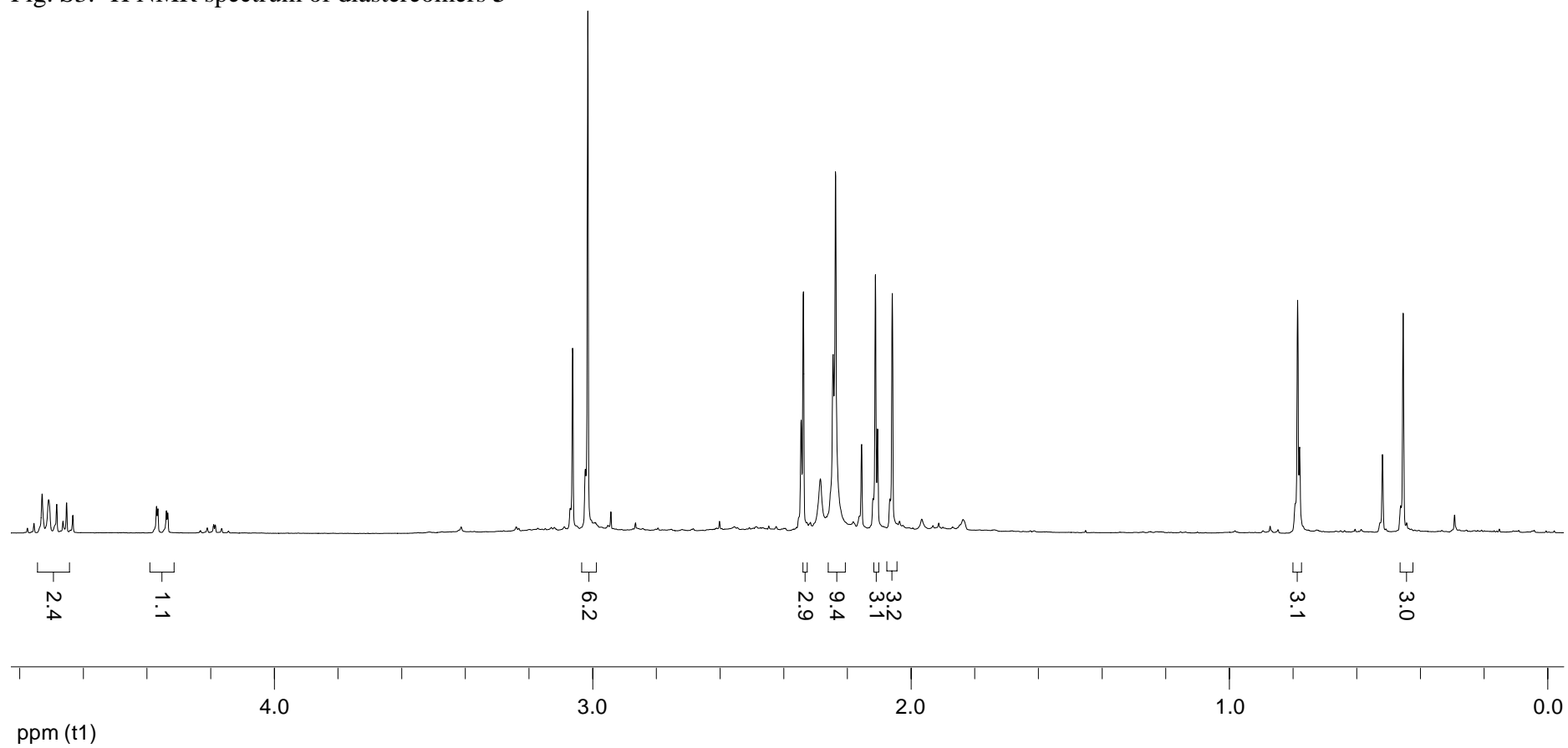
Fig. S3. ^1\text{H} NMR spectrum of diastereomers 3
