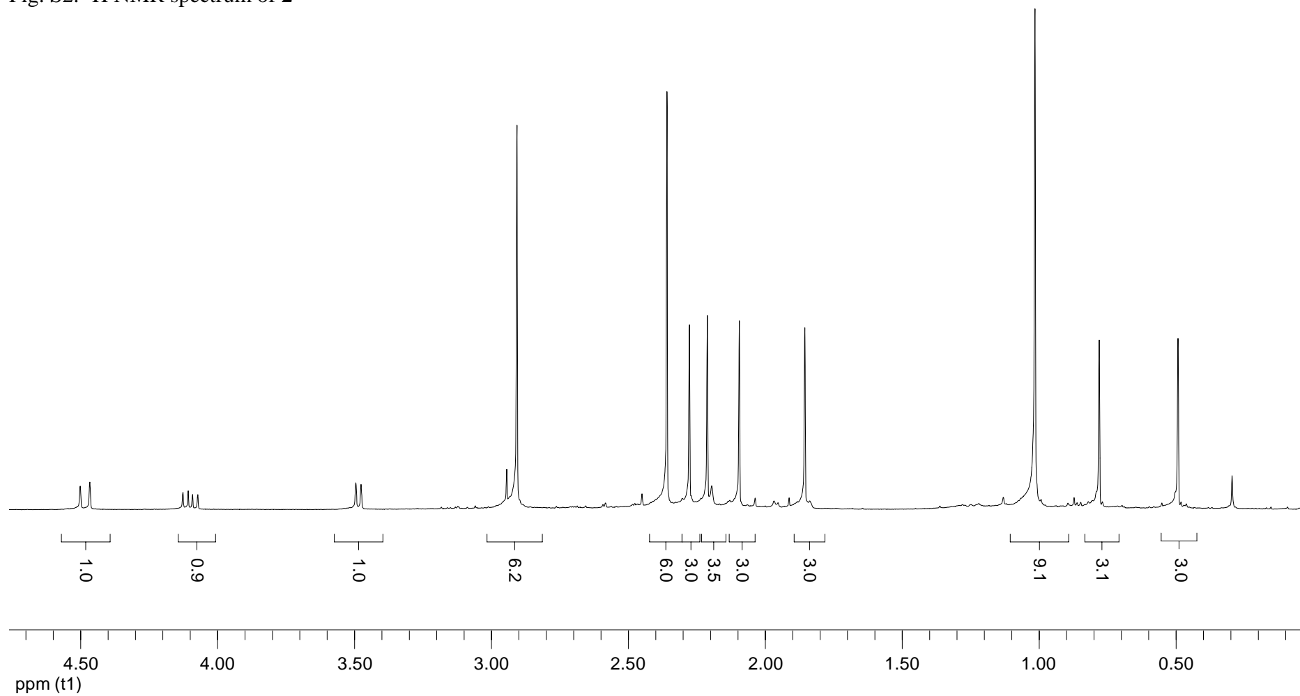
Fig. S2. ^1\text{H} NMR spectrum of 2
