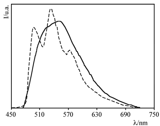
FIGURE S3 - Luminescence spectra of 8 in acetonitrile fluid solution at 298 K (solid) and in butyronitrile rigid matrix at 77 K (dashed).
