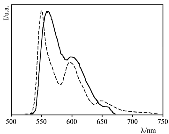
FIGURE S4 - Luminescence spectra of 10 in acetonitrile fluid solution at 298 K (solid) and in butyronitrile rigid matrix at 77 K (dashed).
