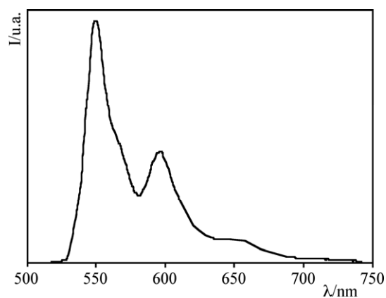
FIGURE S2 - Luminescence spectrum of 6 in butyronitrile rigid matrix at 77 K.
