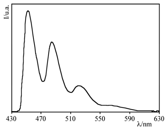
FIGURE S1 - Luminescence spectrum of 1 in butyronitrile rigid matrix at 77 K.
