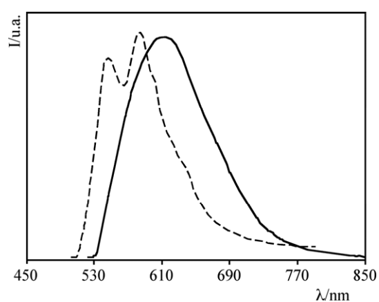
FIGURE S5 - Luminescence spectra of 11 in acetonitrile fluid solution at 298 K (solid) and in butyronitrile rigid matrix at 77 K (dashed).
