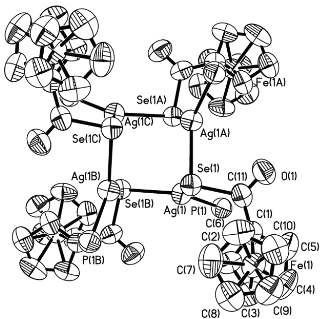
Fig. S1. Molecular structure of (\text{Ph}_3\text{P})_4\text{Ag}_4(\text{Se}(\text{O})\text{CFc})_4 5. Phenyl rings and hydrogen atoms have been omitted for clarity. Thermal ellipsoids are drawn at 40 % probability.
