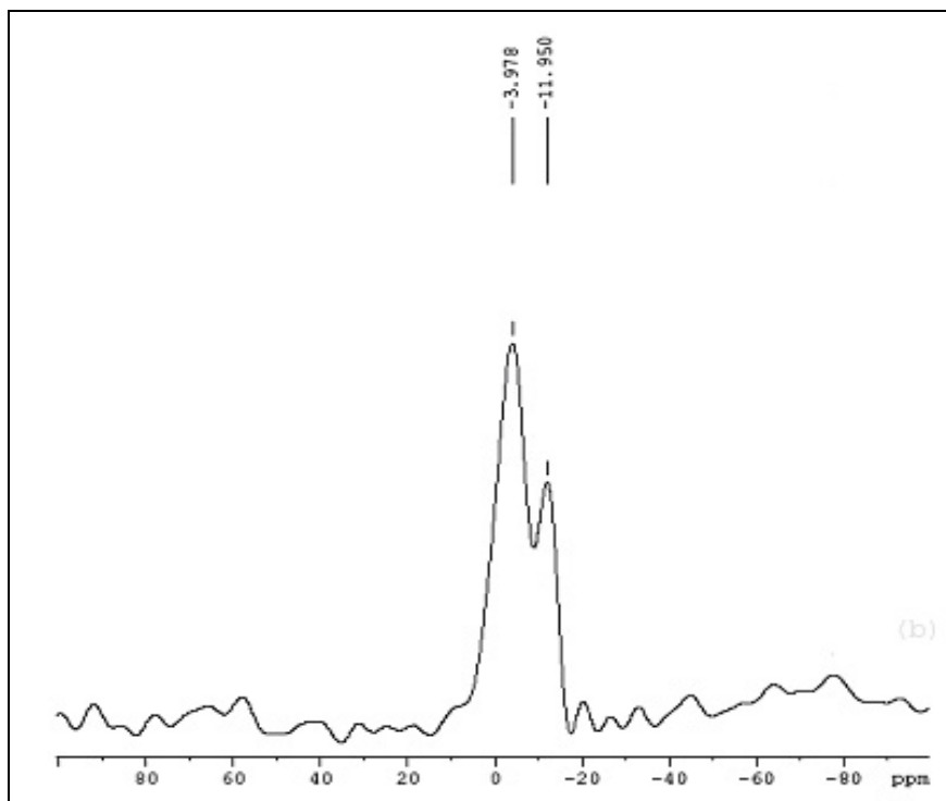
Fig S5 (b) ^{31}\text{P} MAS NMR of \text{LPW}_2/\text{ZrO}_2
