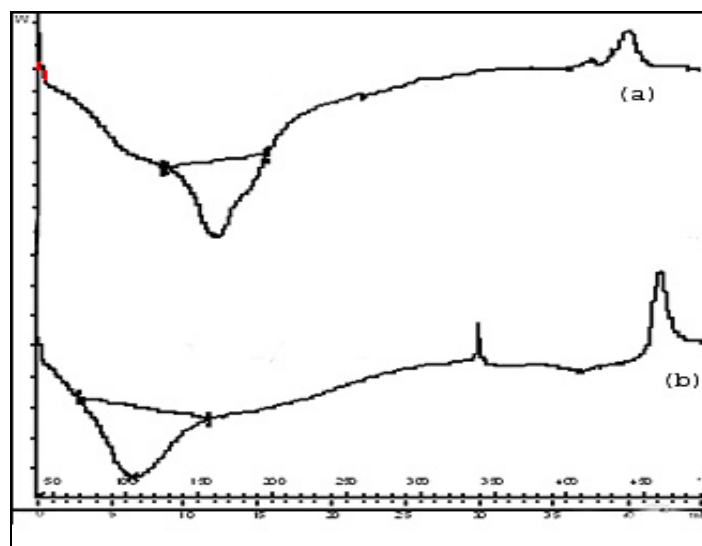
Fig S2 DSC curve of (a) LPW and (b) LPW 2 /ZrO 2
