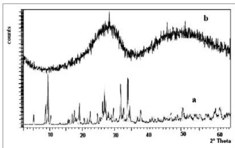
Fig. S6 XRD diffraction pattern of (a) LPW (b) LPW 2 /ZrO 2
