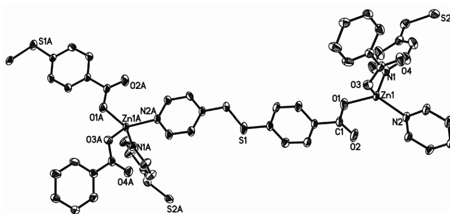
Figure S2 ORTEP plot with numbering scheme for 2
