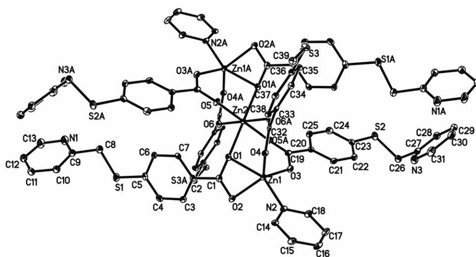
Figure S1 ORTEP plot with numbering scheme for 1
