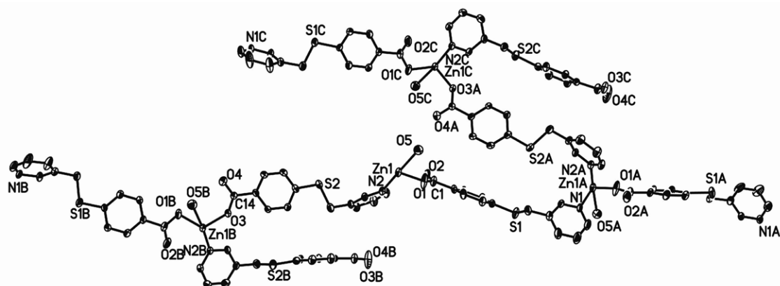
Figure S3 ORTEP plot with numbering scheme for 3
