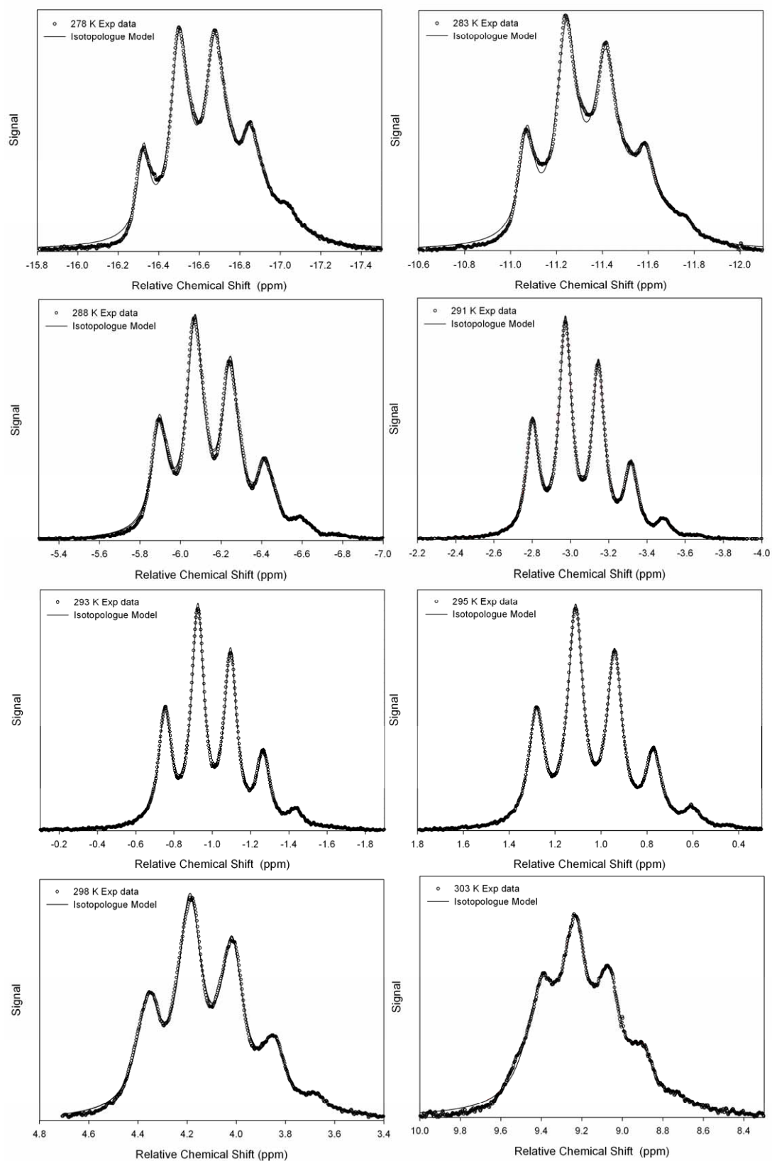
ESI Fig.S1 ^{195}\text{Pt} NMR spectra of [\text{PtCl}_6]^{2-} , for solution II, as a function of temperature. Symbols represent experimental data whereas solid lines represent the least squares fit obtained between the isotopologue model and the experimental data.
