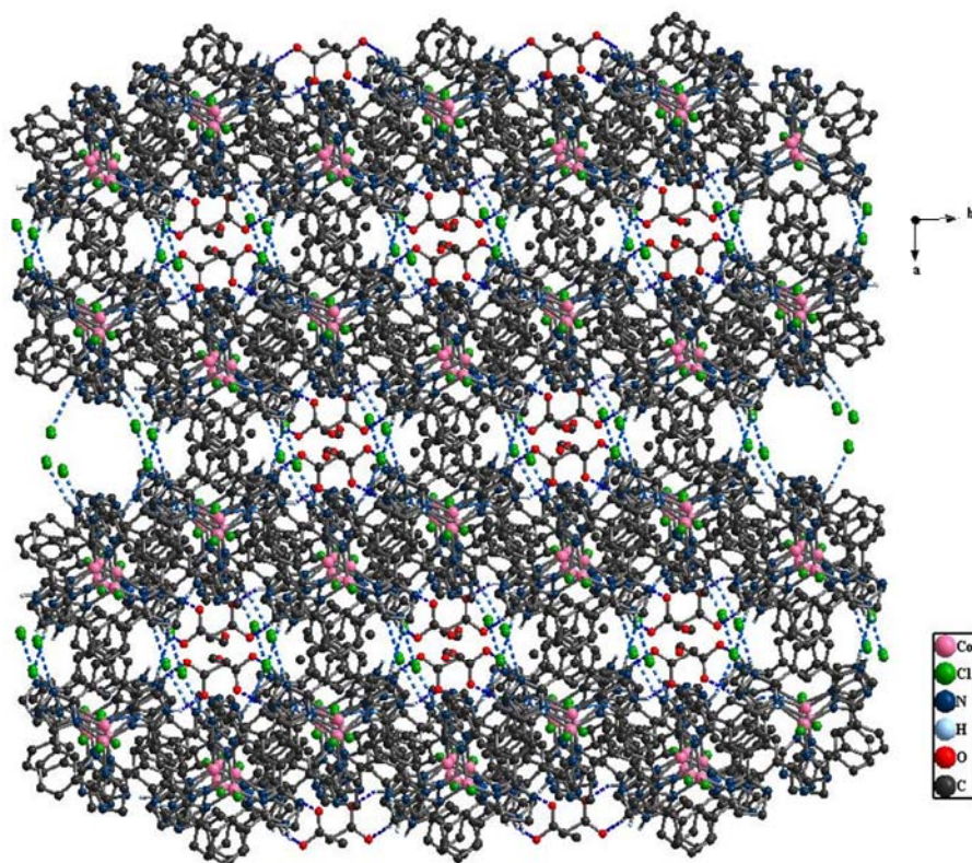
Figure s1 3-D supramolecular networks of 1
