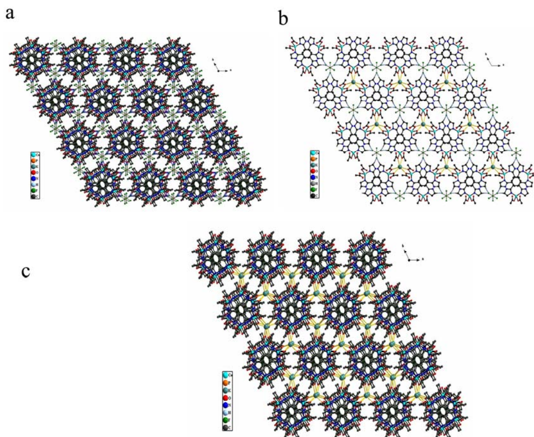
Figure s3 (a) packing of the 3D structure (no containing K^+ ) (b) packing of the 2D layers (c) packing of the 3D structure for 3
