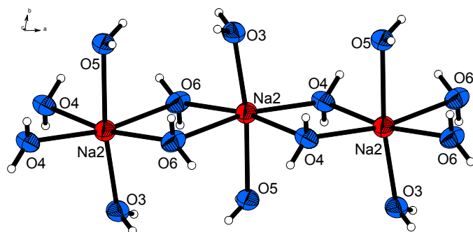
Section of the chain of edge-sharing [Na(2)O 6 ] octahedra running along [1 0 0]. Thermal ellipsoids drawn to 50% probability level.
