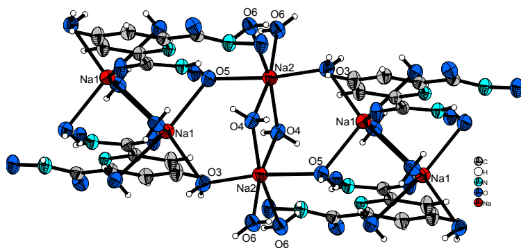
Section of [Na(2)O 6 ] chain with coordinated [Na(1)O 6 ] octahedra pairs. Thermal ellipsoids drawn to 50% probability level.
