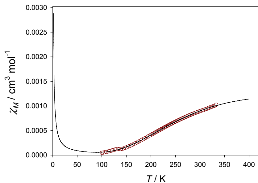
Fig. S2 Thermal dependence of the molar magnetic susceptibility for compound 4 . The solid line is the best fit to the equation (1).
