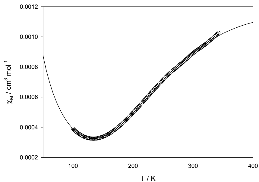
Fig. S1 Thermal dependence of the molar magnetic susceptibility for compound 3 . The solid line is the best fit to the equation (1).
