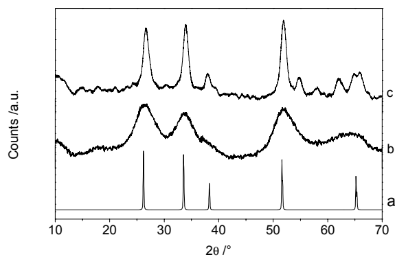
Fig. S1. X-ray diffraction pattern of (a) cassiterite \text{SnO}_2 (JCPDS no.41-1445), (b) \text{S1}_{\text{Br}} , (c) \text{S1}_{\text{Br}}^{550}
