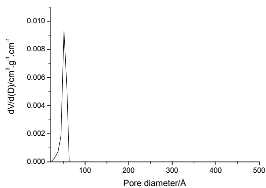
Fig. S2. Pore size distribution of \text{S2}_{\text{TFSI}}^{550}
