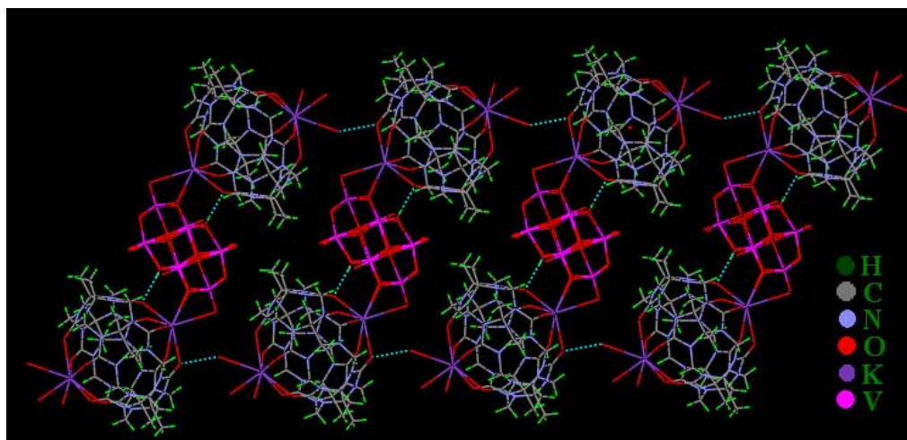
Figure 2S. A view showing sandwich-type subunit to form 1D supramolecular strap based on H-bonds (in dashed line) in 2
