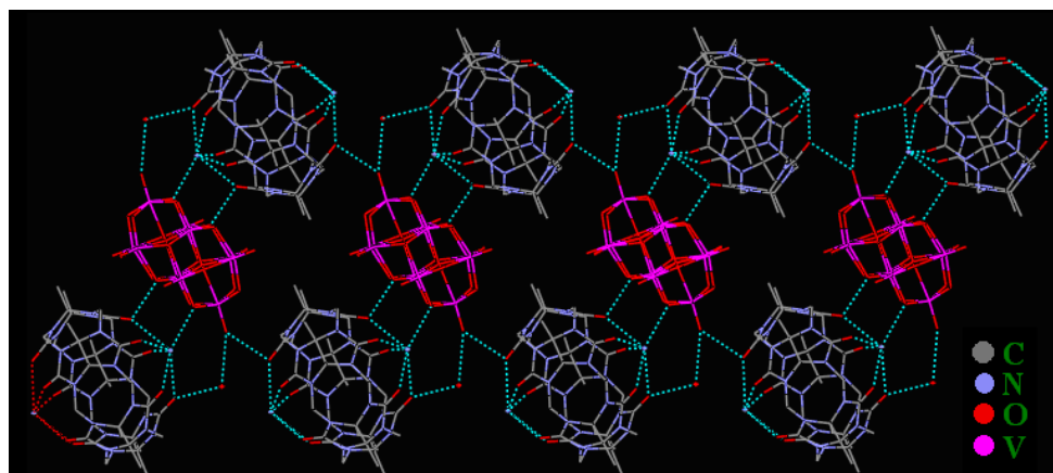
Figure 1S. Supramolecular cingulum constructed from the sandwich-type units through hydrogen bonding interaction in 1
