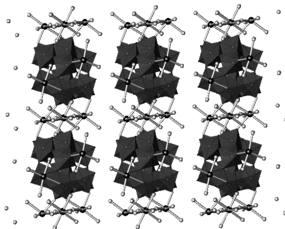
Figure 1-Structure of Na 5 [H 7 W 12 O 42 ]·20H 2 O looking down the c -axis, where WO 6 are shown as grey polyhedra and sodium cations and oxygen atoms both as black spheres.
