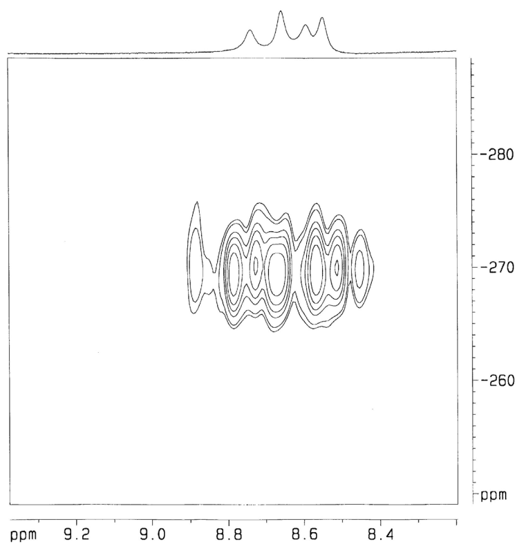
Figure A. ^{15}\text{N} - ^1\text{H} HMBC spectrum of 1b (lower field, evolution time 5.5 msec) in \text{CDCl}_3 at 25^\circ\text{C} .
