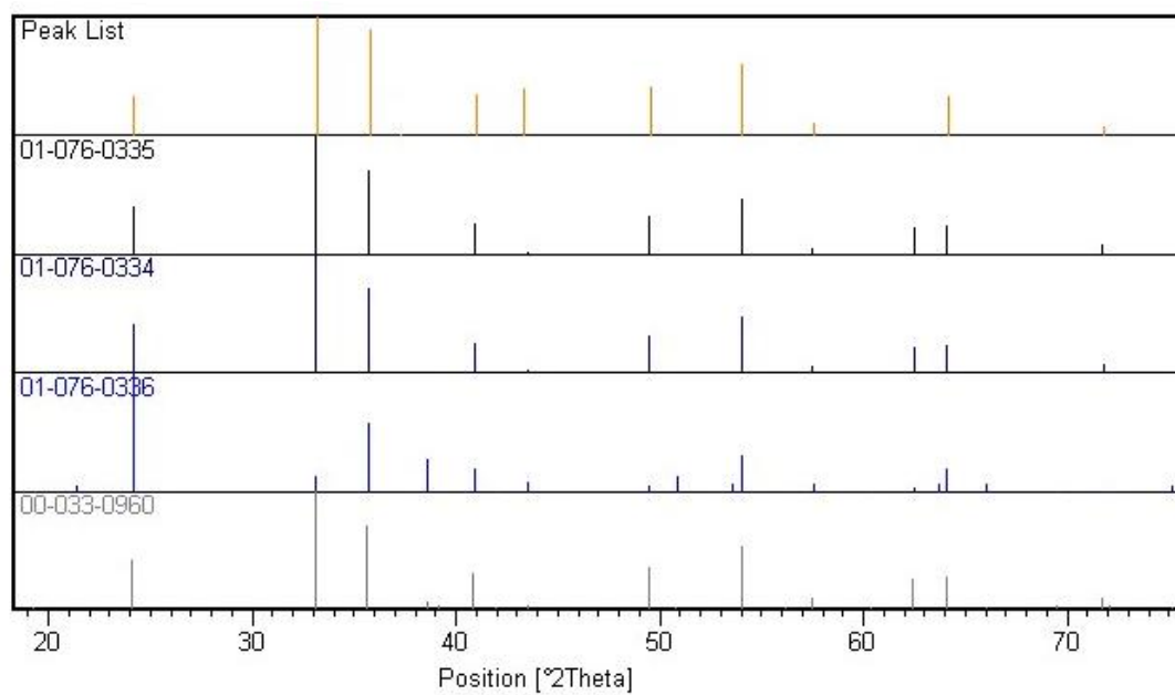
Figure 7: Comparison of XRD pattern of \text{NiTiO}_3 thin film deposited from complex (1) with standard ICCD cards of \text{NiTiO}_3 .
