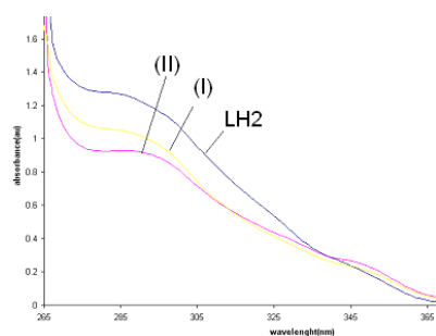
Supplementary Figure : UV-visible spectra of LH2 with Ar = phenyl, I and II each of them in dimethylformamide( 10^{-3} M)
