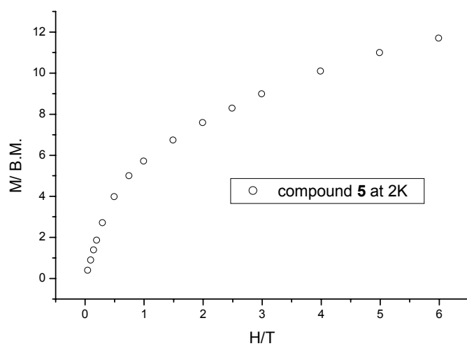
Fig. S5. M vs H for compound 5 at 2 K
