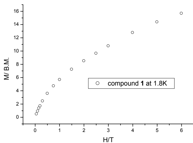
Fig S1. M vs H for compound 1 measured at 1.8 K.
