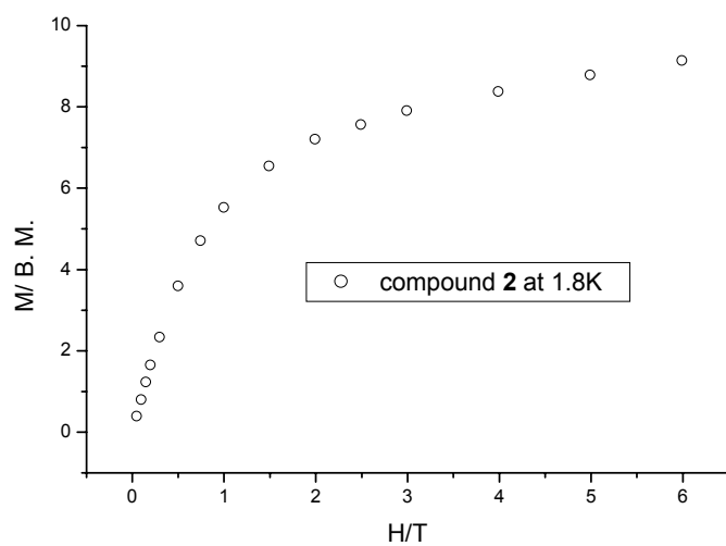
Fig S2. M vs H for compound 2 measured at 1.8 K
