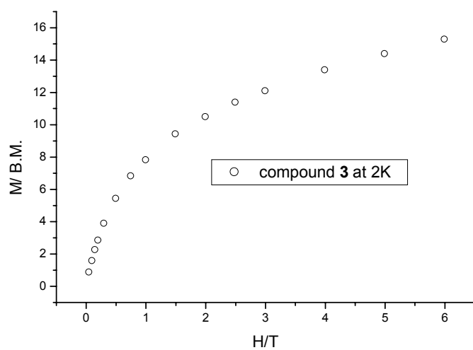
Fig. S3. M vs H for compound 3 at 2 K.
