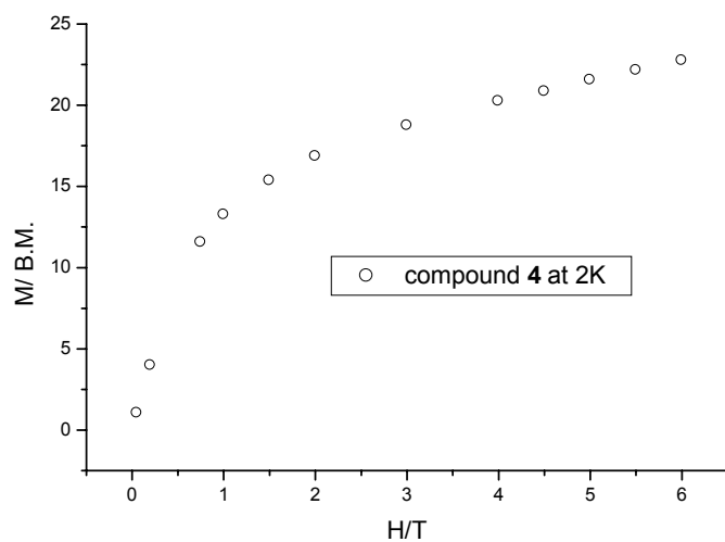
Fig. S4. M vs H for compound 4 at 2 K.
