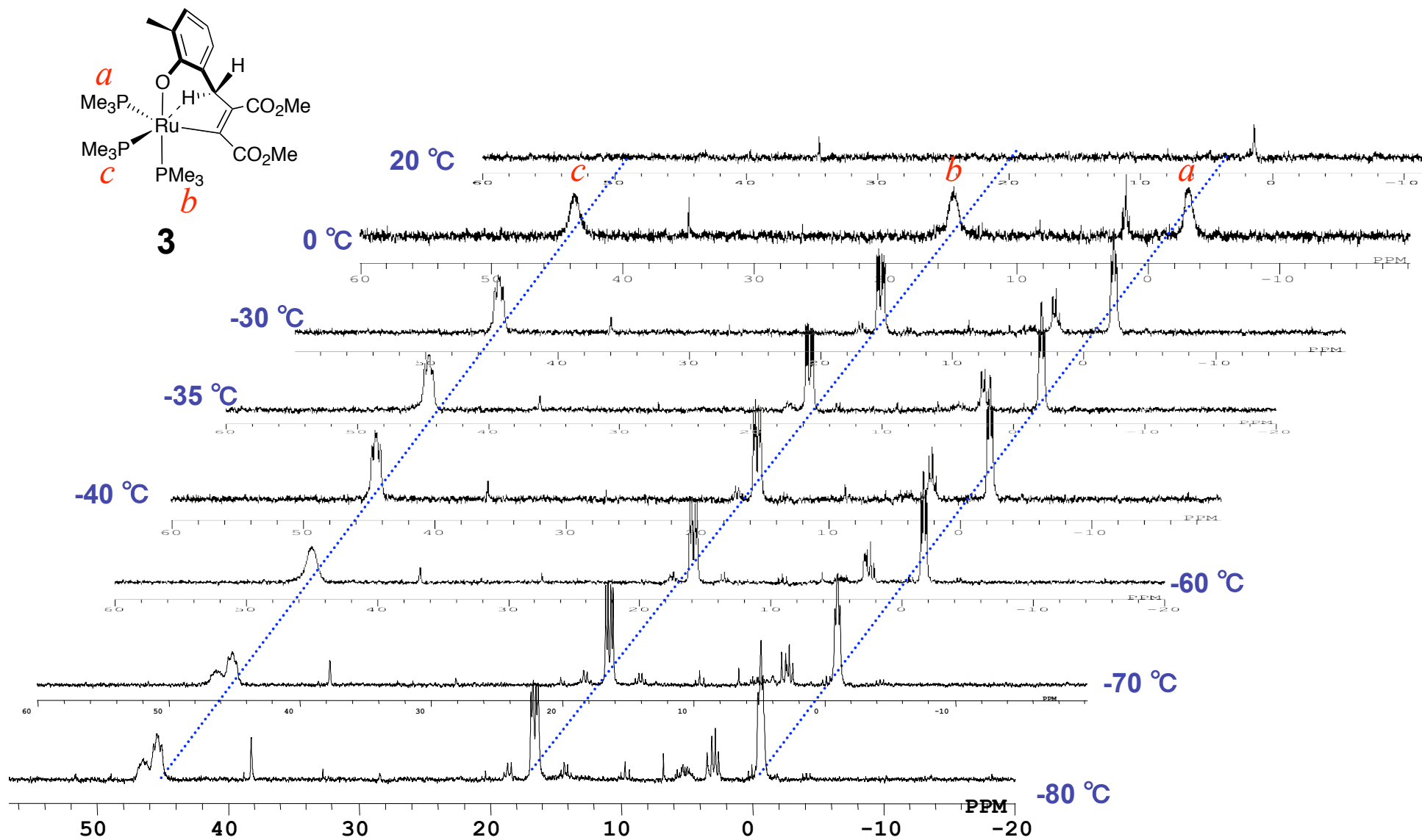
Fig.S1. Variable-temperature ^{31}\text{P}\{^1\text{H}\} NMR spectra of 3 in acetone- d_6 .
