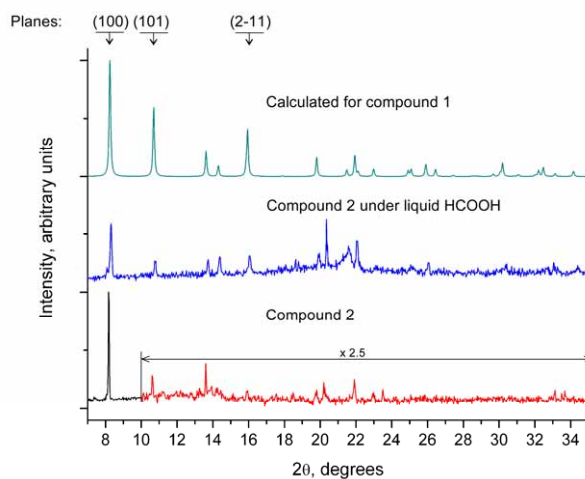
Figure S2. Powder XRD of 2 , 2 with formic acid and calculated XRD for 1 (all for CuK \alpha radiation)
