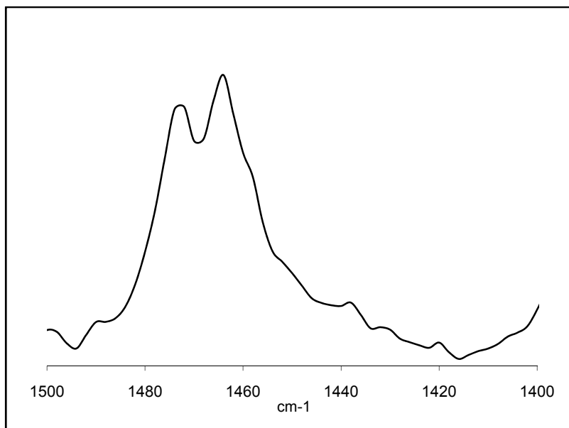
Infrared spectrum of 5 (part)
