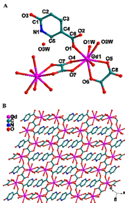
Fig. S2. Coordination environment of Gd1 atom in 4(A) and 2D framework of 4(B).
