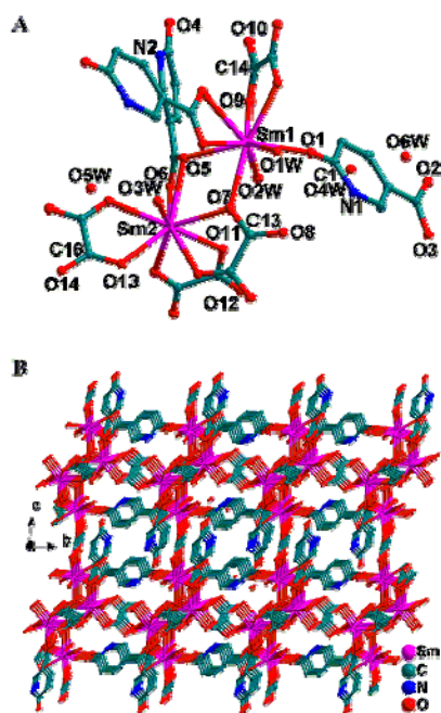
Fig. S1. Coordination environment of Sm atoms in 2(A) and 3D framework of 2 viewed along the a -axis (B).
