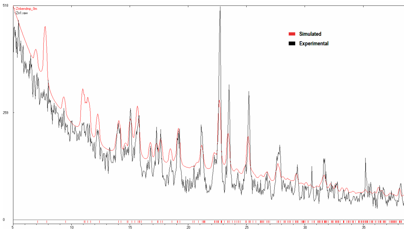
Fig: Simulated and experimental PXRD patterns for Complex 1
