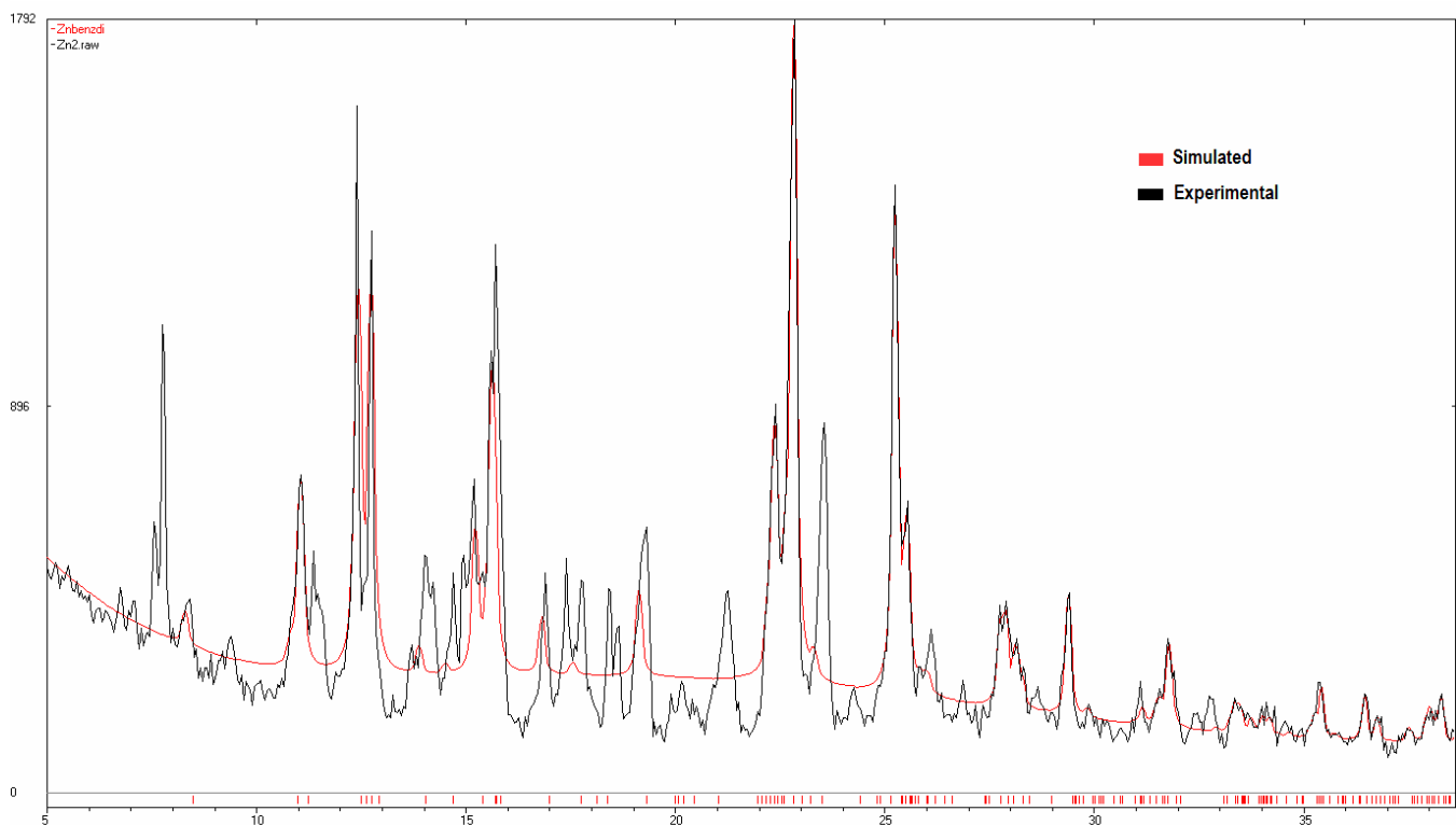
Fig: Simulated and experimental PXRD patterns for Complex 2
