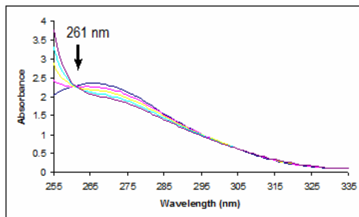
Fig: Ultraviolet absorption spectra of complex 6 in methanol ( 10^{-3} M) upon addition of dimethylformamide (100 \mu l per aliquot).
