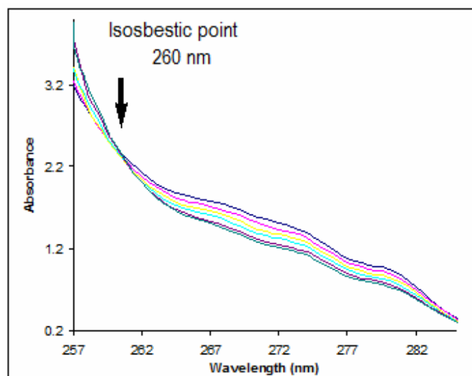
Fig: Ultraviolet absorption spectra of complex 3 in methanol ( 10^{-3} M) upon addition of dimethylformamide (100 \mu l per aliquot).
