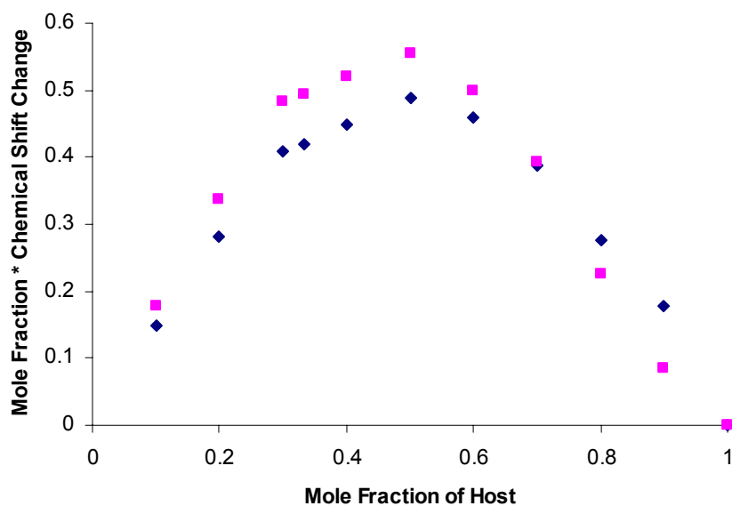
Fig. S2: Job plot for L and \text{NBu}_4^+\text{OAc}^- in \text{DMSO-}d_6 solution.
