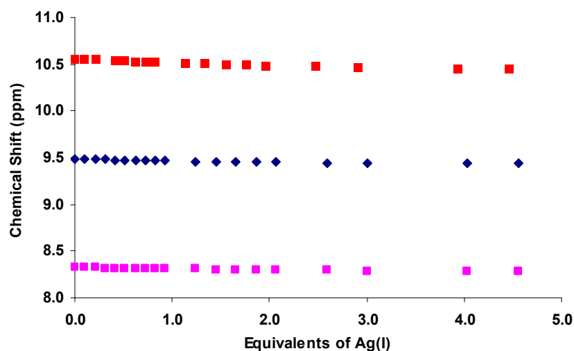
Fig. S1: Titration of L with \text{AgCF}_3\text{SO}_3 in DMSO solution.
