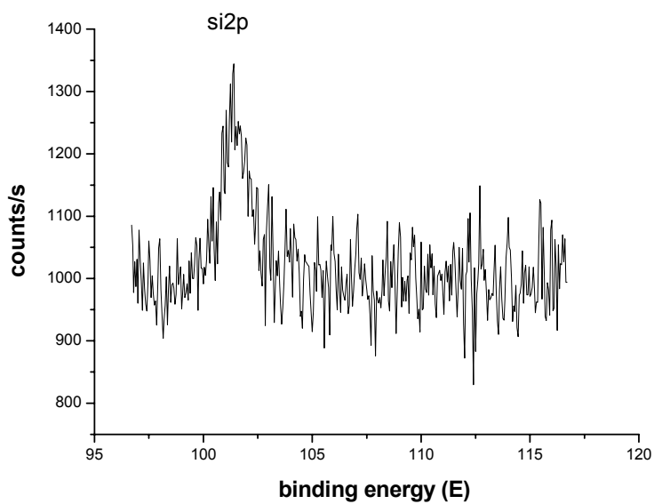
Fig S1. The XPS spectrum of the Si2p region of compound 1 .
