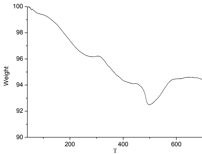
Fig s4, The TG curve of compound 1.
