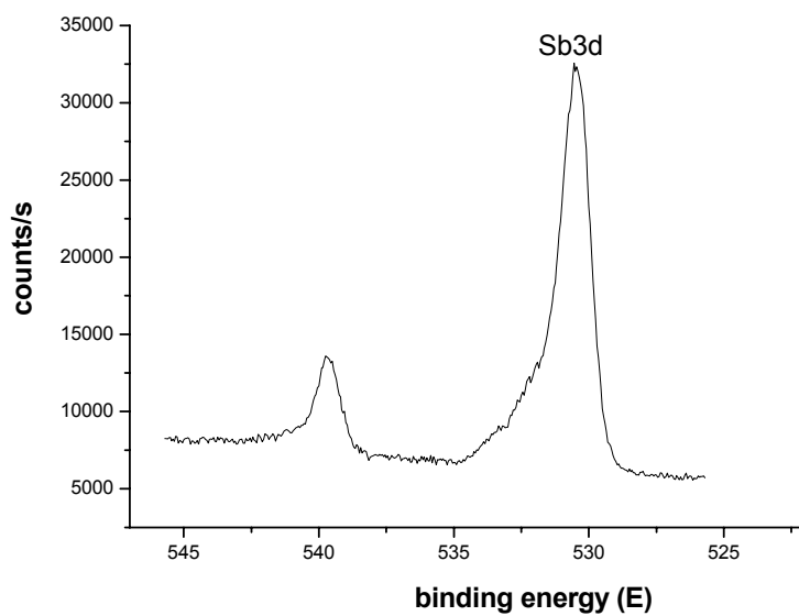
Fig S2. The XPS spectrum of the Sb3d region of compound 1 .
