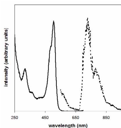
Figure S3. Emission (dotted line) and excitation (solid line) spectra of complex 8 in CH 2 Cl 2 at 77K.
