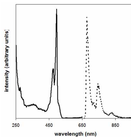
Figure S2. Emission (dotted line) and excitation (solid line) spectra of complex 7 in CH 2 Cl 2 at 77K.
