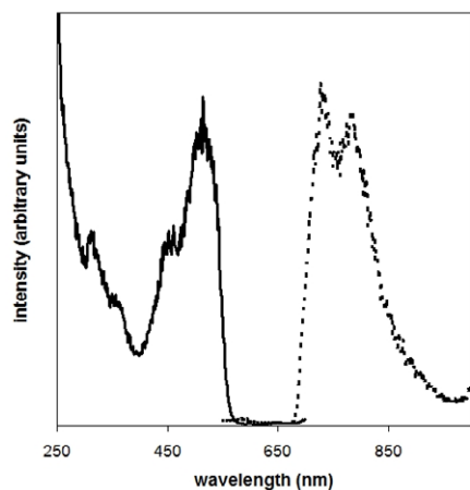
Figure S1. Emission (dotted line) and excitation (solid line) spectra of complex 6 in CH 2 Cl 2 at 77K.
