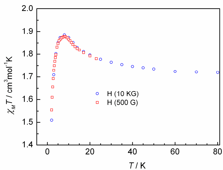
Figure S3: Plots of \chi_M T vs. T at applied magnetic field of 500G and 10KG for 1 .
