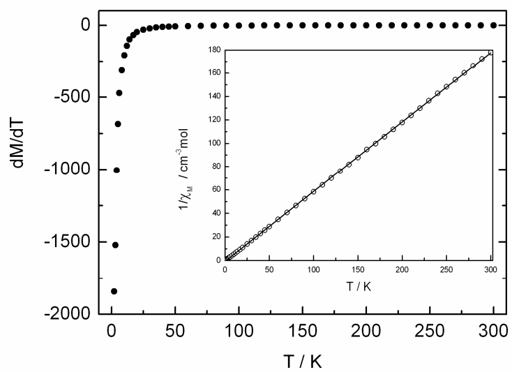
Figure S2: Plots of dM/dT vs. T and (\chi_M)^{-1} vs. T (inset) for 1 .
