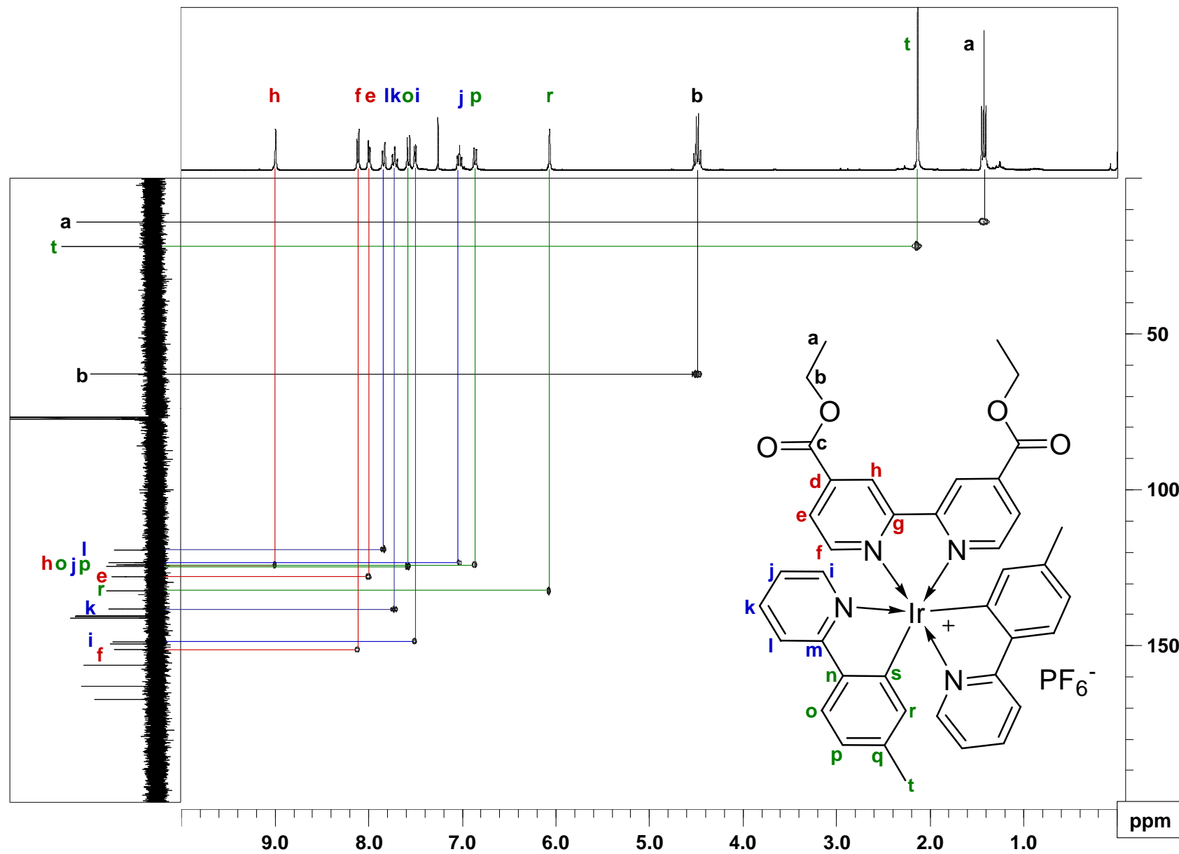
Figure S4. HSQC of complex 1.
