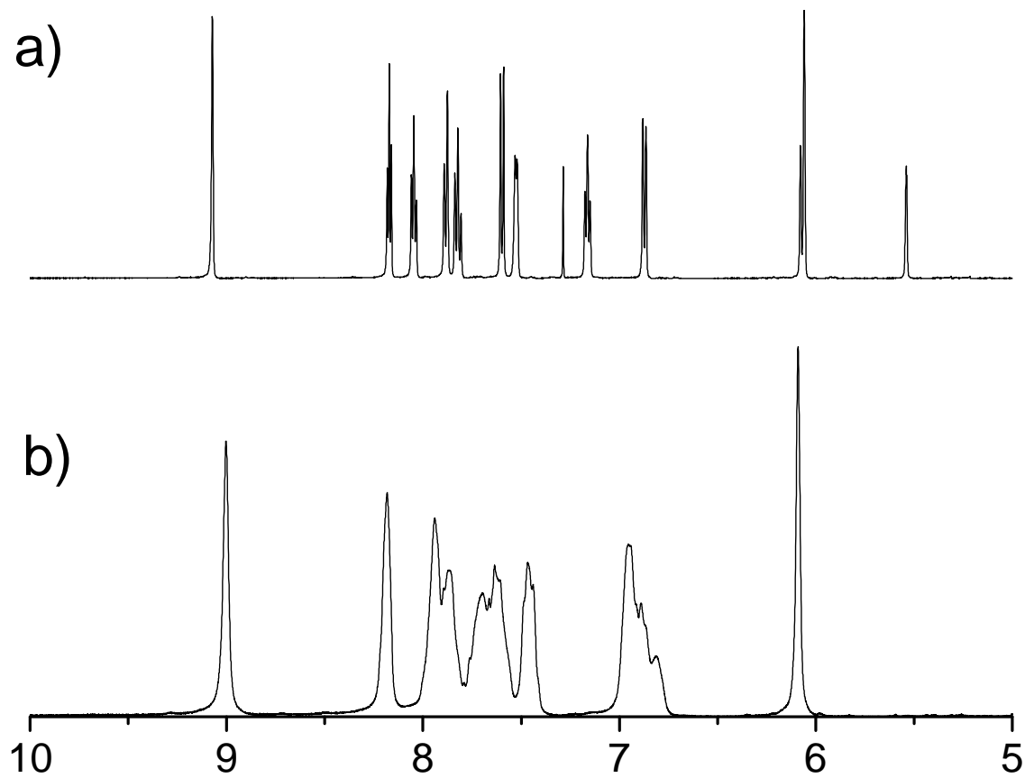
Figure S1. a) 1 H-NMR in CDCl 3 of the monomer 7 and b) 1 H-NMR in CD 2 Cl 2 of the polymer 2 .
