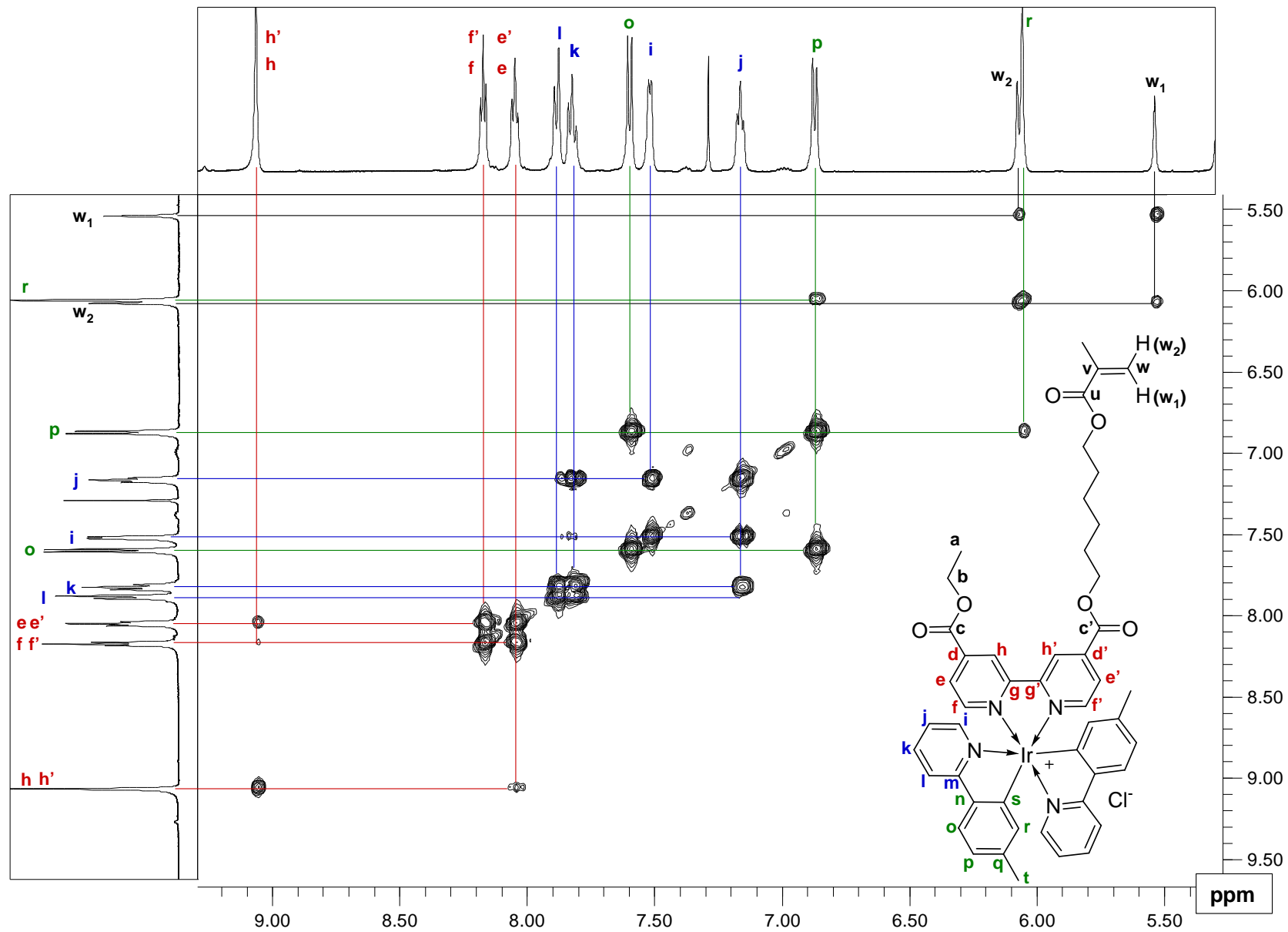
Figure S2. DQF-COSY of monomer 7.
