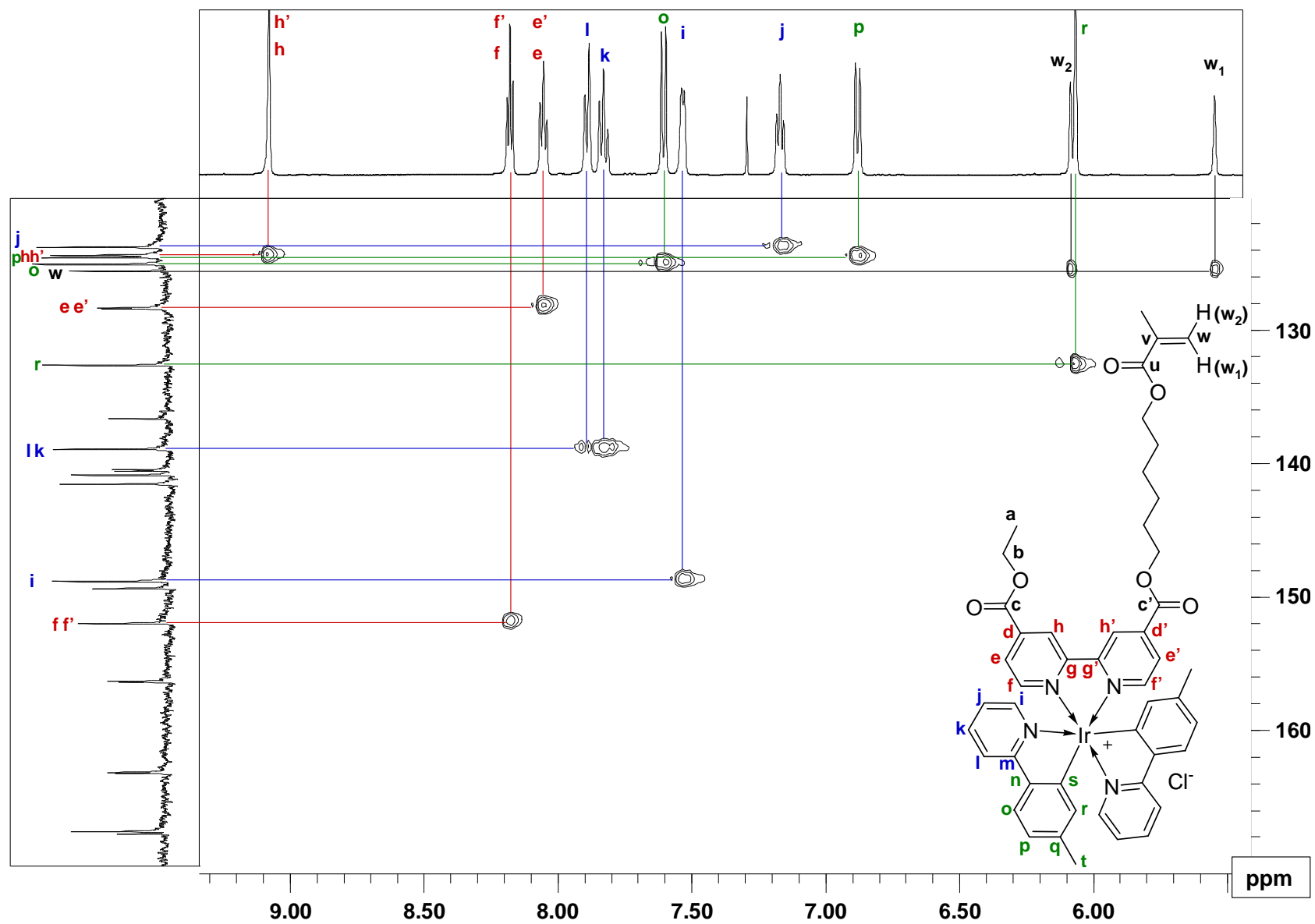
Figure S3. HSQC of monomer 7.
