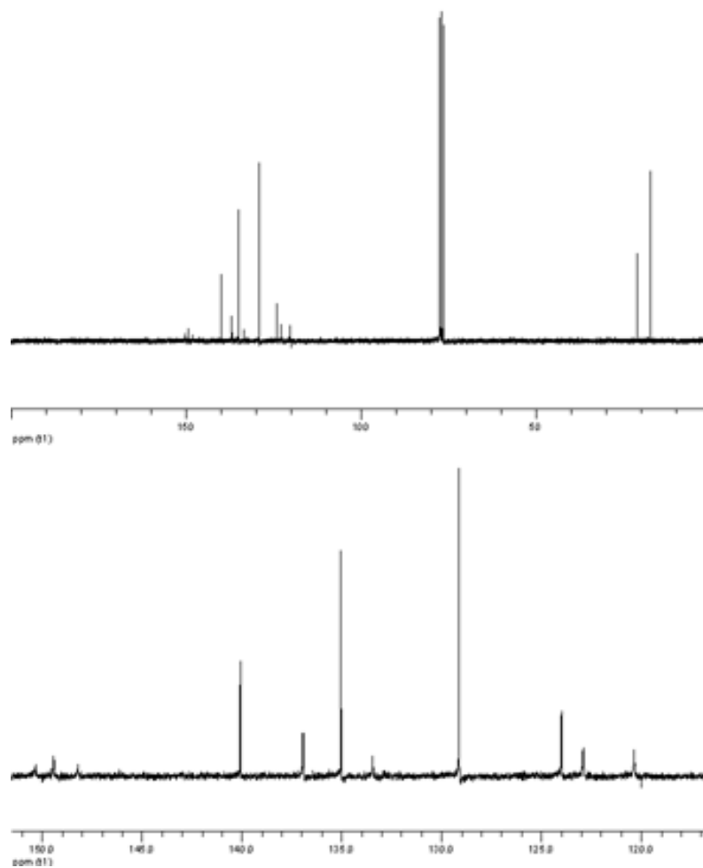
Fig. S2: ^{13}\text{C} NMR spectrum of 2 in \text{CDCl}_3 , top: full range, bottom: selected range.
