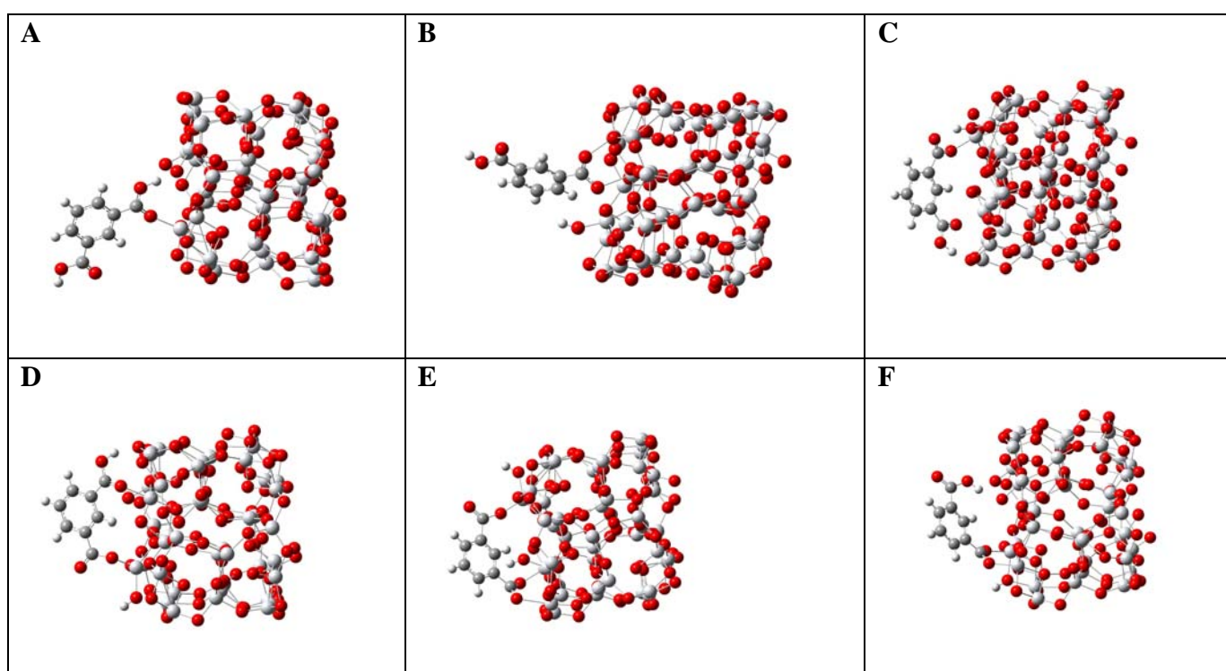
Figure ESI1. Fully optimized binding modes A – F of Ipa to (TiO 2 ) 46 .
