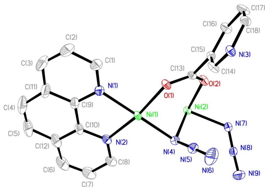
Fig. S1 The asymmetric unit of 1
