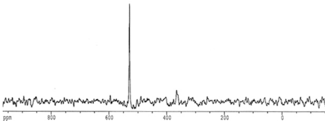
Fig. S1 ^{113}\text{Cd} NMR spectrum for 1 .
