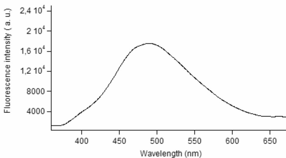
Fig. S2 Fluorescence emission spectrum for 1 ( 2 \times 10^{-5} M) measured in acetonitrile ( \lambda_{\text{exc}} = 350 nm).
